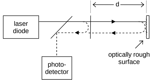
Figure 4. Observation of interferometric speckle in an in-line configuration.
