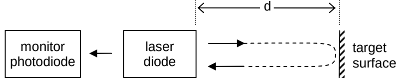
Figure 1. Typical schematic configuration for measurement of deflection using laser diode self-mixing. After Guiliani et al [4] .
