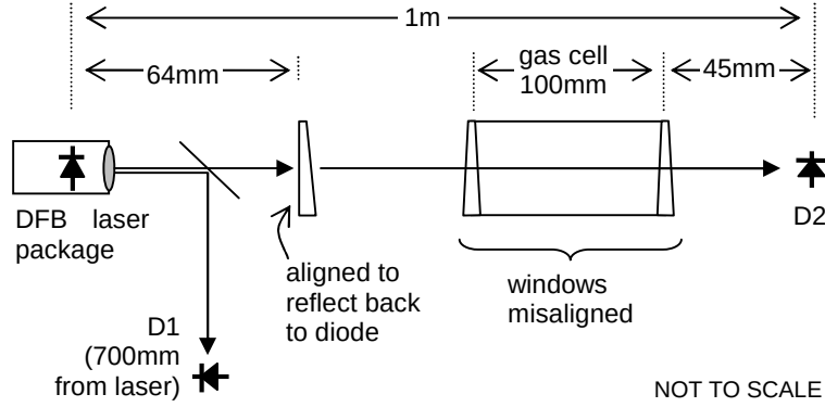
Figure 15. Configuration of experiments to investigate self-mixing feedback in gas absorption measurements.
