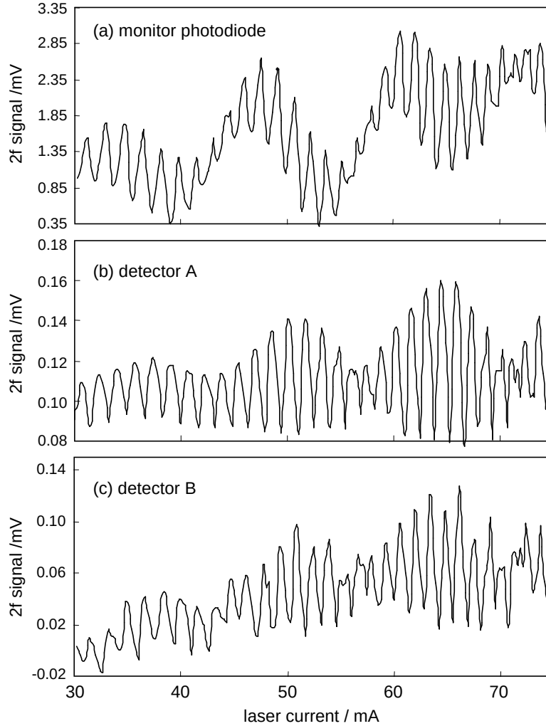
Figure 9. Interferometric signals caused by feedback from a wedged window placed 154mm from the laser, obtained at (a) the reference photodiode (100k \Omega transimpedance gain), (b) detector A (0dB gain), (c) detector B (30dB gain). The laser temperature was set to 40° (away from the gas line). Note different scales.
