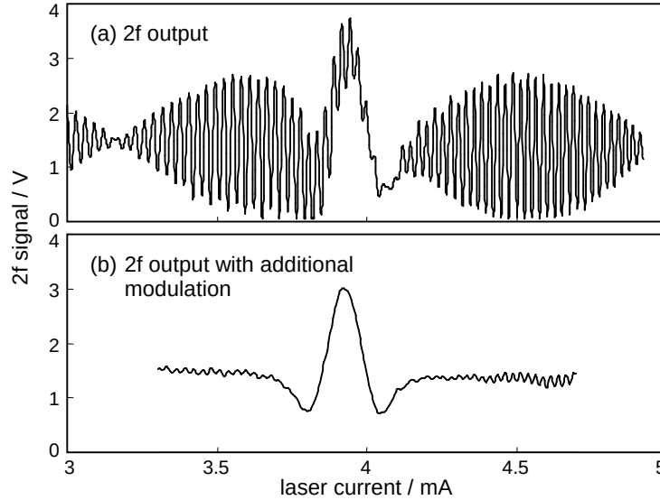
Figure 18. 2f WMS signals acquired by the microLGD TM for a methane concentration of 100ppm.
