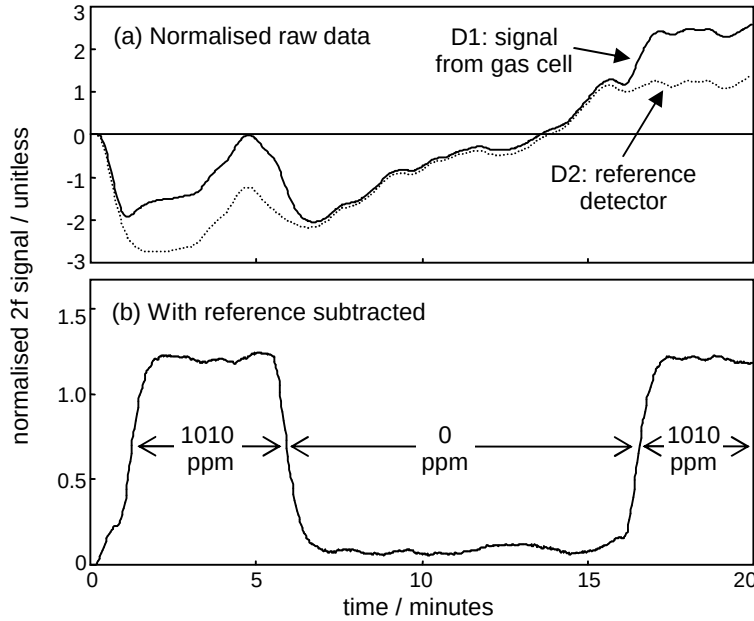
Figure 17. Normalised 2f-demodulated output from detectors D1 and D2 plotted as a time series while different methane concentrations (in air) were delivered to the gas cell. (a) Normalised raw data, (b) data corrected by subtraction of the reference. (Lock-in \tau 10s.)
