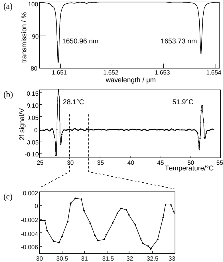
Figure 7 (a) Theoretical methane transmission lines obtained from the Hitran database [8] for a pathlength of 5.3mm. (b) 2f signals obtained from the monitor diode while temperature tuning the laser. (c) Expansion of (b). The fringe spacing was approximately 1\pm0.2 \text{ } ^\circ\text{C} , corresponding to a cavity spacing of 12\pm2 \text{ mm} .
