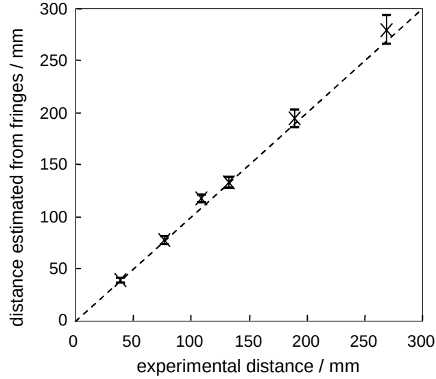
Figure 13. Results of self-mixing feedback from a diffuse reflector: distance estimated from the fringe count versus measured experimental distance from reflector to laser diode.
