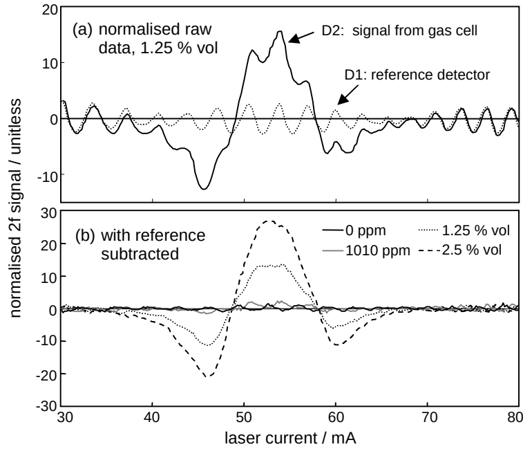
Figure 16. Results of wavelength scans through a methane line at different concentrations, while high levels of feedback were deliberately applied to the laser diode. (a) Normalised 2f signal components, (b) signals from D2 corrected by subtraction of the reference signal from D1. (Lock-in \tau 100ms.)
