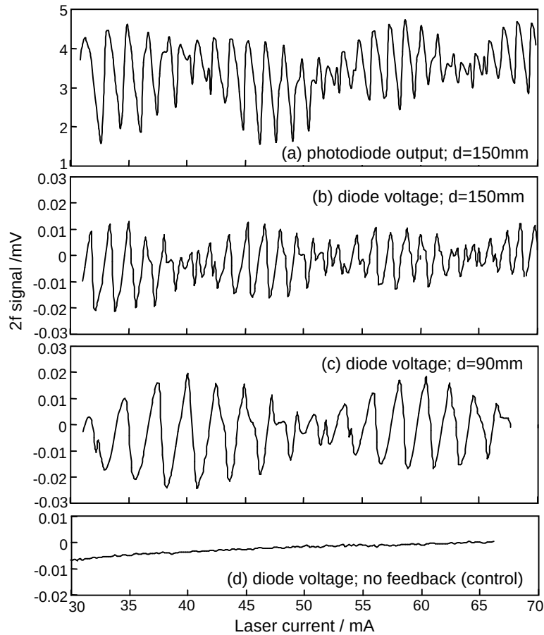
Figure 11. Comparison of the self-mixing – induced 2f signal components (a) on the laser monitor photodiode, (b), (c) on the laser diode voltage, and (d) on the laser diode voltage in a control experiment with no external feedback.
