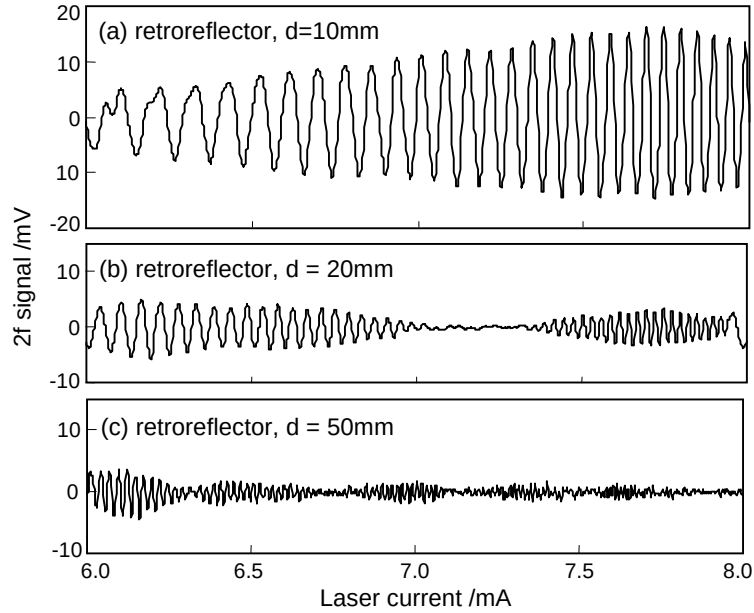
Figure 14. Self-mixing interference observed as a modulation of the voltage across a VCSEL. Second harmonic signals obtained with retroreflective tape placed at distance d of (a) 10mm, (b) 20mm and (c) 50mm.
