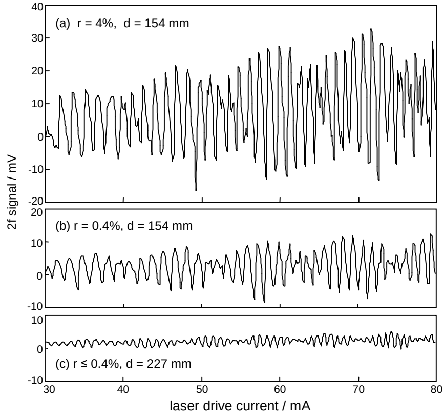
Figure 10. Self-mixing induced interference fringes observed in the laser diode forward emission for feedback from (a) an uncoated 6° wedged window at a distance of 154mm, (b) an AR coated 6° wedged window at a distance of 154 mm, and (c) the latter at a distance of 227 mm.
