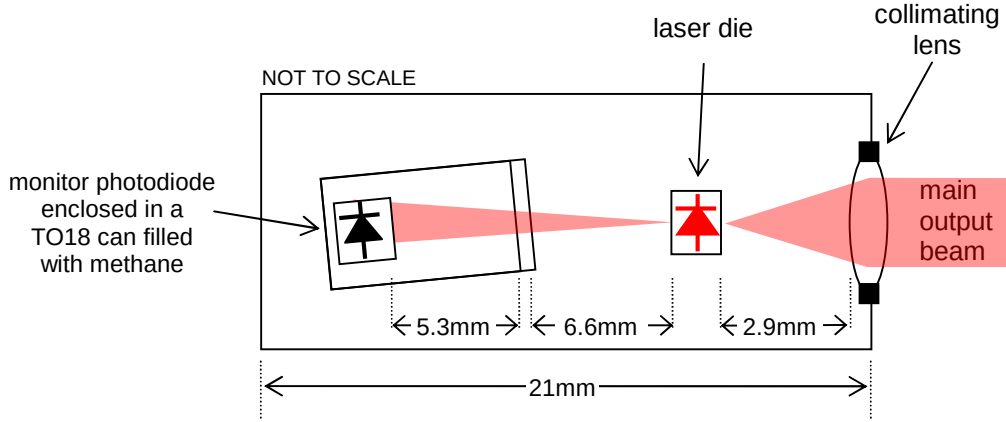
Figure 6. Optical layout of the DFB laser package, showing key distances between components.
