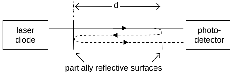
Figure 3. A low-finesse etalon in the optical path of a detection system; the partially reflective surfaces are often the windows of the gas sample cell.
