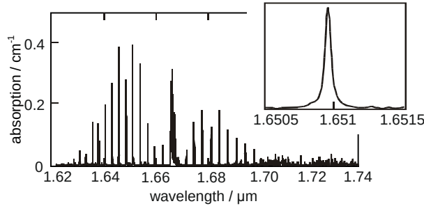
Figure 2. Absorption spectrum for 100% methane in the near infra-red, calculated using data from the HITRAN database [8] .
