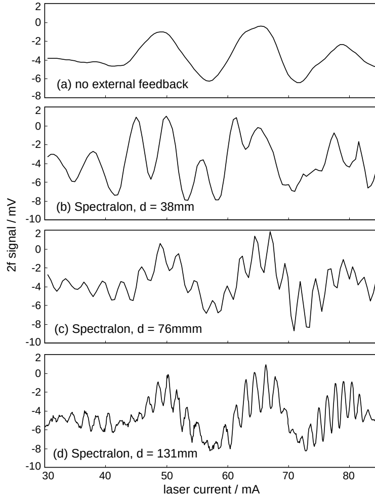
Figure 12. Self-mixing modulation of the output from the rear facing DFB monitor photodiode by feedback from a Spectralon TM plate placed at different distances from the laser. (a) No external feedback, (b) d = 38mm, (c) d = 76mm, (d) d = 131mm.
