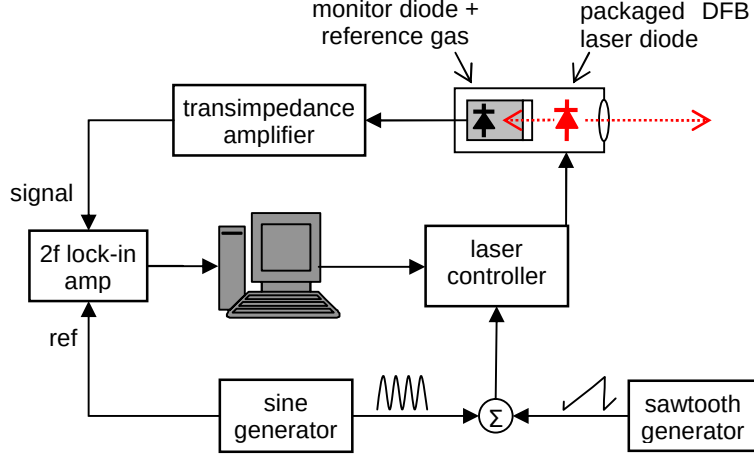
Figure 5. Schematic experimental configuration for 2f wavelength modulation spectroscopy, implemented using the emission from the rear facet of the DFB laser in order to distinguish self-mixing interference from other types of interference.
