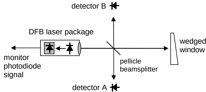
Figure 8. Schematic diagram of the experimental configuration to measure the effects of feedback from a wedged window
