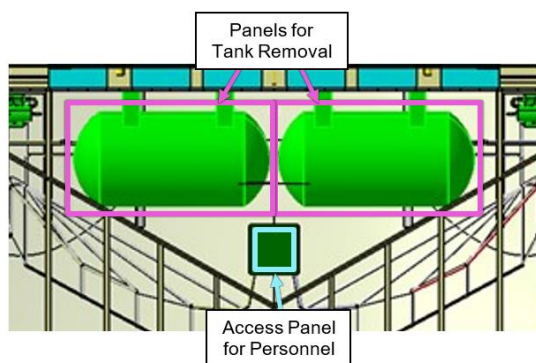
Figure 15. Recommended Locations of Lower Fuselage Panels
