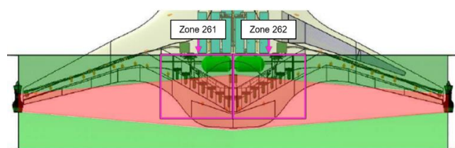
Figure 16. Portions Affected By Engine Rotor Burst (Highlighted in Red) [11]
