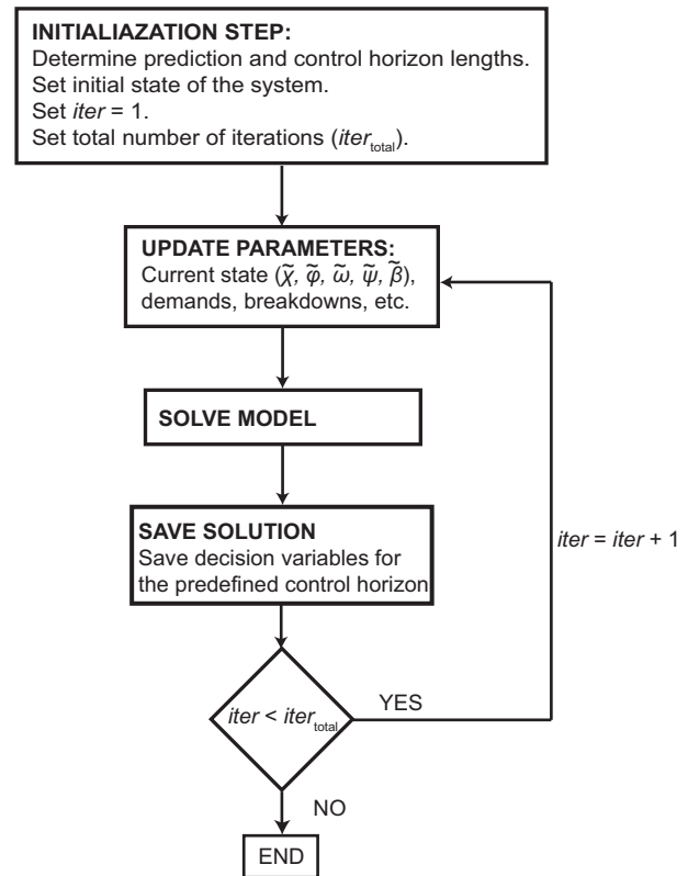
Fig. 7. A representative rolling horizon algorithm.
