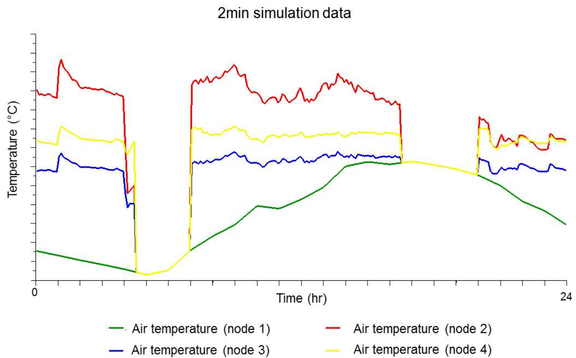
Figure 5. Temperature profiles (relating to Figure 3 flows) - 2min interval data
