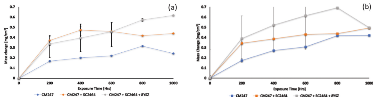
Figure 4. Averaged weight change plot showing mass change vs exposure time for test 1 and 2; (a) Metal change for 800^\circ\text{C}/1 \text{ bar}/\text{CO}_2 + 2.7 \text{ mol}\% \text{ H}_2\text{O} + 0.17 \text{ mol}\% \text{ O}_2 and (b) Metal change for (b) 800^\circ\text{C}/1 \text{ bar}/\text{CO}_2 + 1.43 \text{ mol}\% \text{ N}_2 + 0.17 \text{ mol}\% \text{ O}_2 + 300 \text{ ppm SO}_2 .
