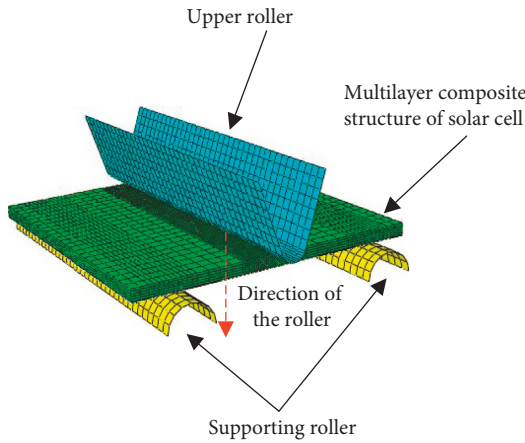
FIGURE 7: The finite element mesh model of the bending test about multilayer composite structure of solar cells.
