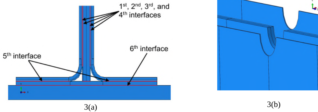
Figure 3: (a) Location of Cohesive Zone Modelling (CZM) layers highlighted, (b) modelled dent on the stiffener web
