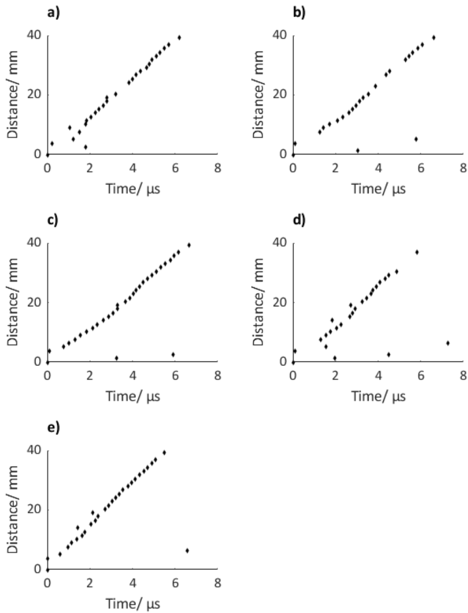
Figure 5. Distance (mm) against time ( \mu\text{s} ) for the five cuboid samples detonated, a) Sample A, b) Sample B, c) Sample C, d) Sample D, and e) Sample E.
