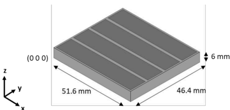
Figure 1. Schematic of the completed print of four cuboids at once. Dark grey shows the bound parts, light grey shows supporting material.
