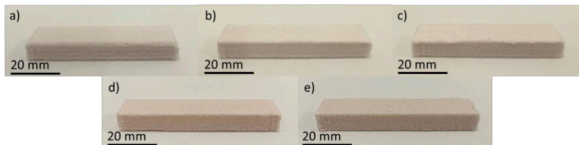
Figure 2. Sample cuboids A to E used to determine the detonation velocity of dry powder printed RDX.
