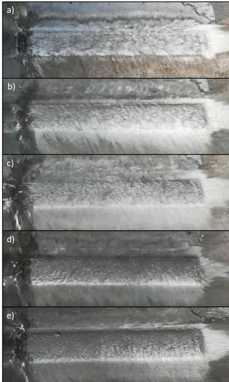
Figure 7. Mild steel (8 mm thickness) witness plates from the five detonation tests, a) Sample A, b) Sample B, c) Sample C, d) Sample and e) Sample E.
