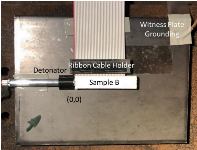
95 Figure 3. Typical set up for the detonation of printed RDX cuboids, where the witness plate 96 is grounded allowing circuit completion when the detonation wave passes.
