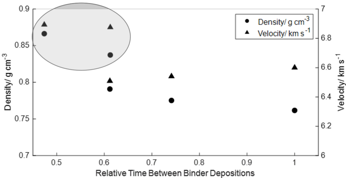
Figure 6. Density (circle) and velocity (triangle) against the relative time between binder depositions, data points from the two-part print inside the highlighted oval.
