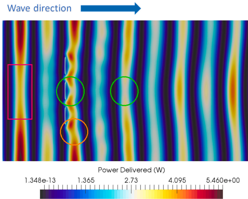
Fig. 8. Plan view of a section of the NWT; the incident wave is from the left side of the plot. Snapshot at 16 s, showing the power delivered by the wave during the performance of the in-line configuration, CG1, when the devices are close and the system is operating destructively (for T_1 ).
