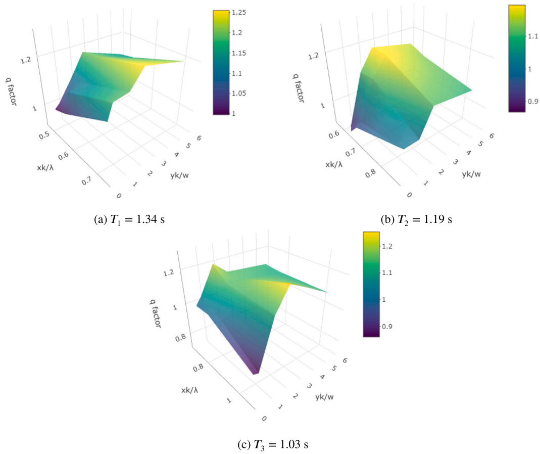
Fig. 18. Surface plots showing the variation of the q factor estimated for layout CG3 operating under different periods. The interaction factor is shown in terms of the non-dimensional distances x_k/\lambda and y_k/w .
