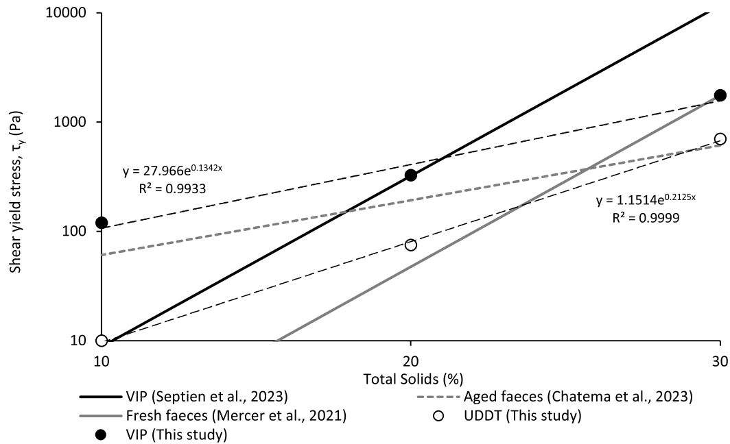
Fig. 7. Yield stress values at ambient temperature for UDDT and VIP sludges, fresh faeces and aged faeces.
