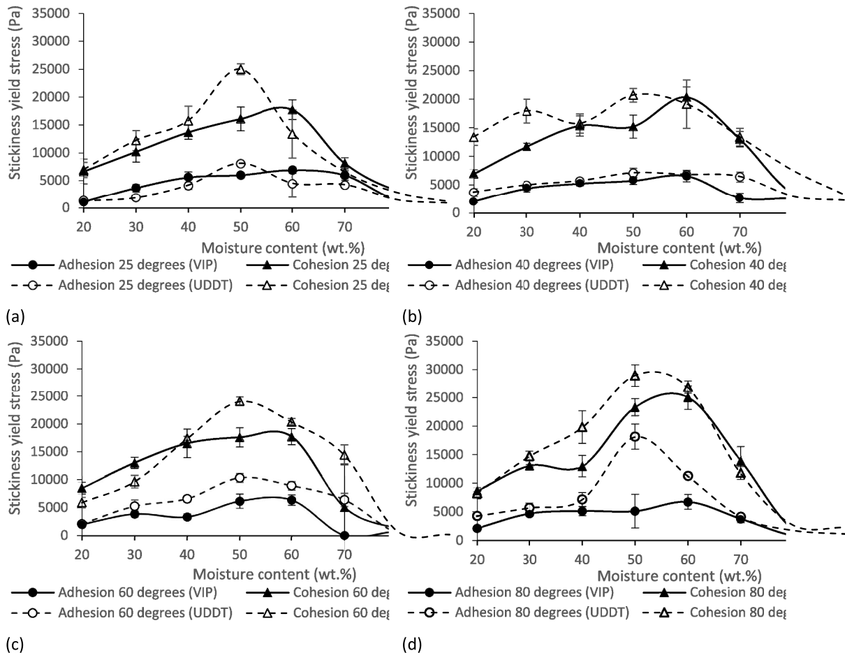
Fig. 2. Impact of moisture content on the adhesive and cohesive stickiness yield stress of VIP and UDDT FS at (a) 25 °C, (b) 40 °C, (c) 60 °C and (d) 80 °C.
