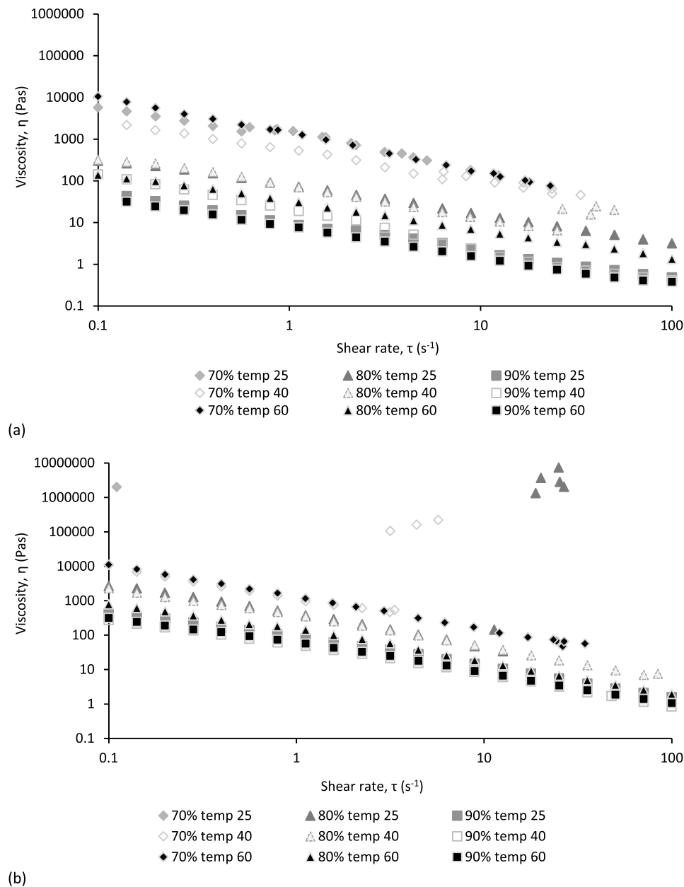
Fig. 6. Viscosity as a function of shear rate at varying temperatures and moisture contents for (a) UDDT (b) VIP sludge types.
