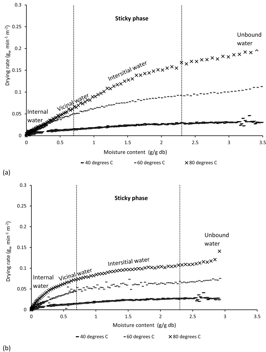
Fig. 5. Drying kinetics at 40 °C, 60 °C and 80 °C of (a) UDDT and (b) VIP sludge types.
