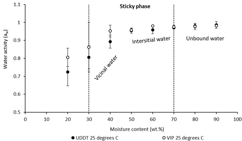
Fig. 4. Characterisation of bound water zones of UDDT and VIP sludge types using water activity measurements at ambient temperature.
