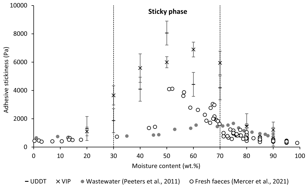
Fig. 3. Comparison of adhesive stickiness at ambient temperature for UDDT FS, VIP FS, wastewater sludge and fresh faeces.
