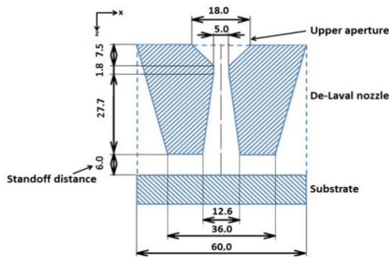
Fig. 3: Nozzle geometry (unit: mm).
