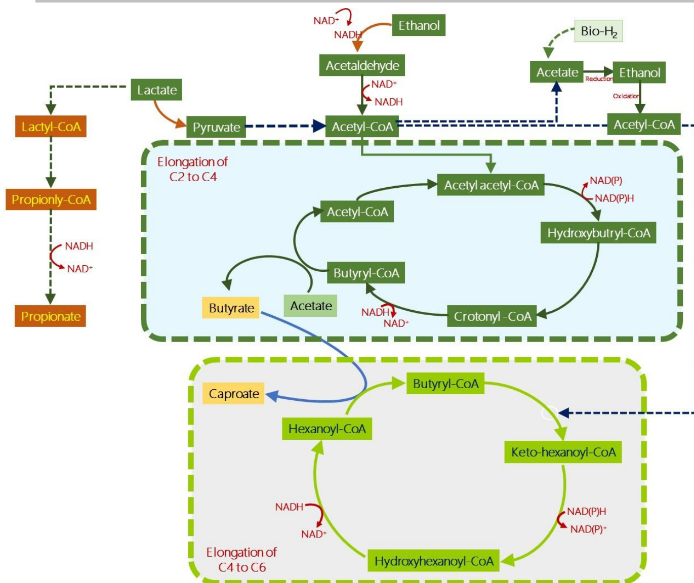
Figure 5: Medium-chain fatty acids production mechanism using bio-hydrogen, lactate, and ethanol as electron donors
