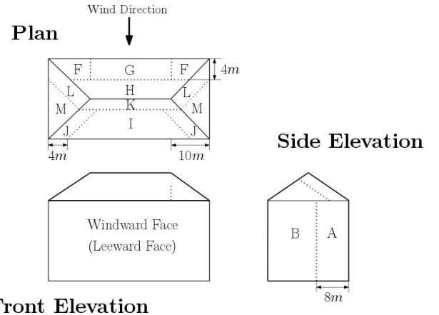
Fig. 3 Building sketch showing the surfaces defined under the BS EN 1991-1-4:2005 + A1:2010 standard used to determine the external pressure coefficients c_{pe}
