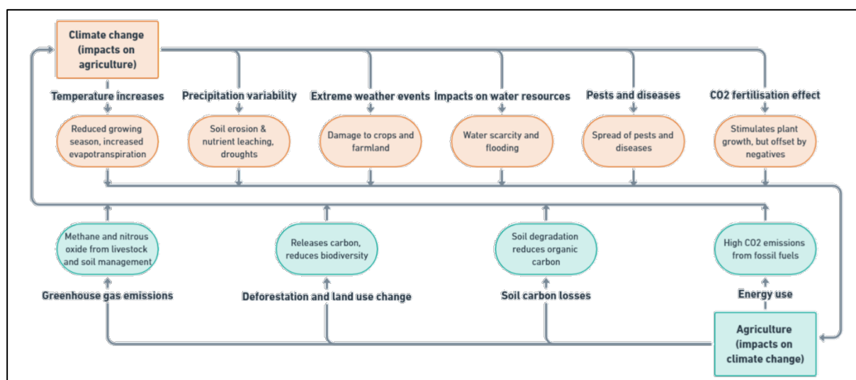
Figure 1. Main interactions between climate change and agriculture
