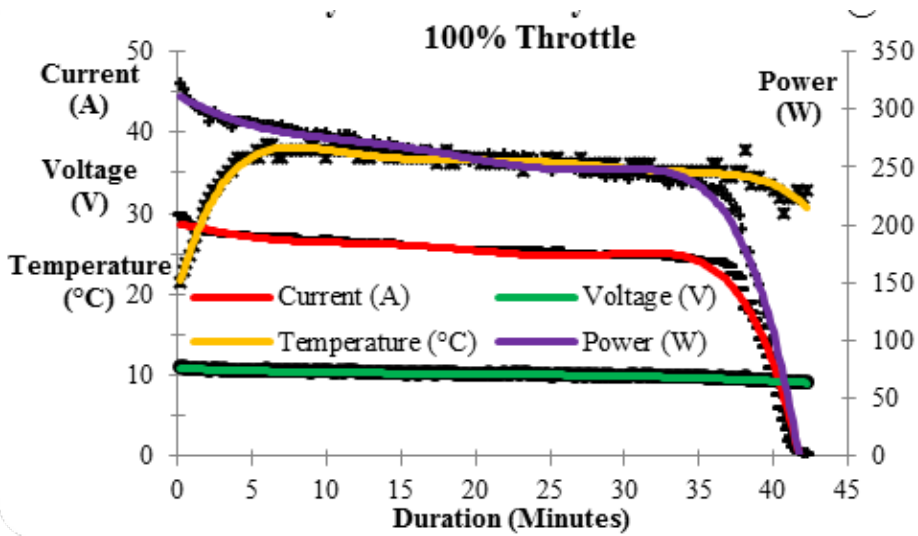
Fig. 5 Prototype UAV's Power Systems - Bench Test @ 100% Throttle
