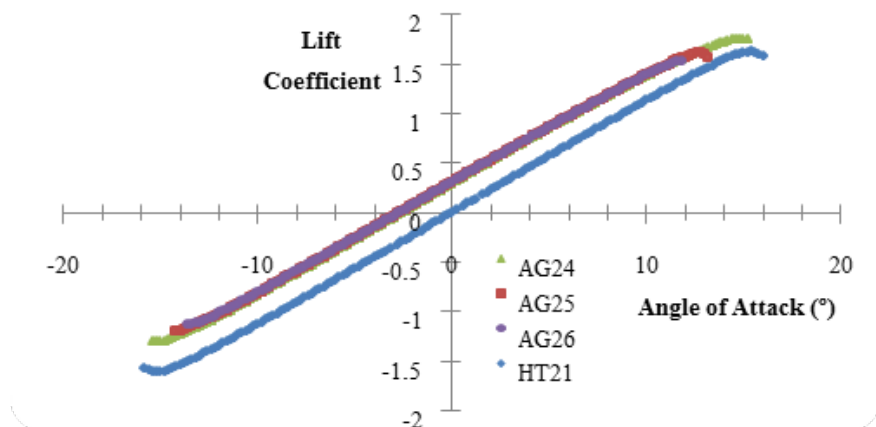
Fig. 2 Lift coefficient versus angle of attack of prototype model airfoils
