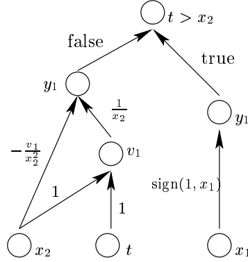
FIGURE 4. The subgraph related to the IF block (supernode)
