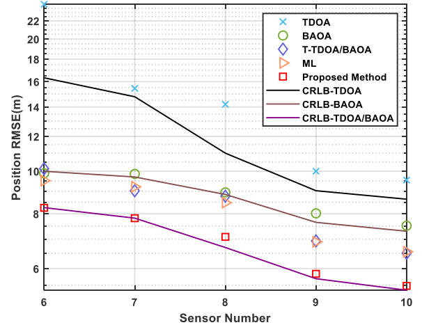
Fig. 11 Comparison of RMSE with different methods.
