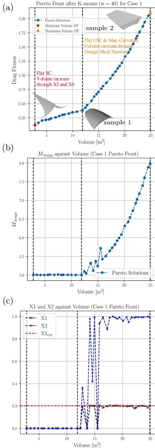
Fig. 10. Pareto front as function of the volume and the drag fitness (a). Pareto front as a function of the volume and the design Mach number (b). Design parameters as functions of the volume indicating two distinct geometries as the results of the optimisation (c).
