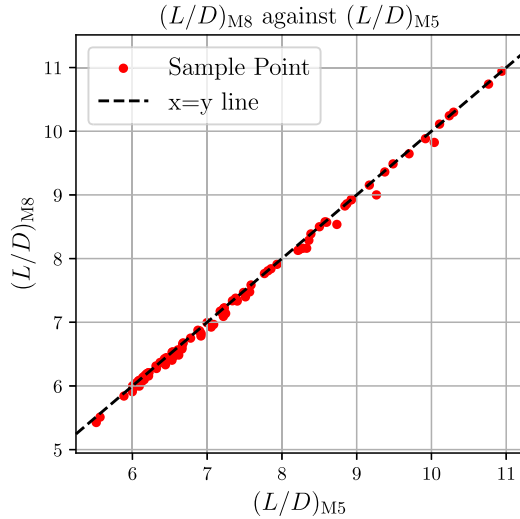
Fig. A.14. Inviscid L/D Mach 5 vs Mach 8 for surrogate samples.
