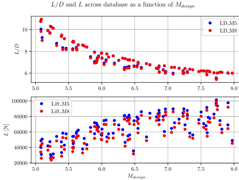
Fig. 12. (L/D)_{M5} , (L/D)_{M8} (top) and L_{M5} , L_{M8} (bottom) as a function of M_{\text{design}} across the sampled points.
