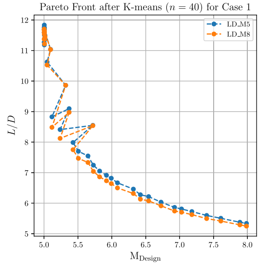
Fig. B.16. L/D as a function of M_{\text{design}} across the optimised geometries.
