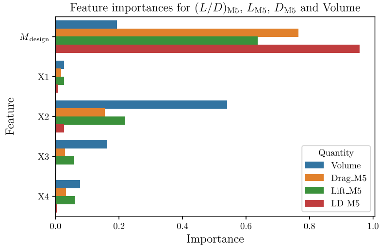
Fig. 8. Feature importances for (L/D)_{M5} , L_{M5} , D_{M5} and volume.
