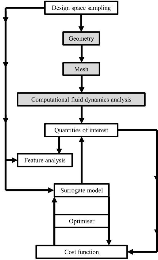
Fig. 1. Schematic of the proposed waverider optimisation framework inspired by the work of Son et al. [31]. The grey boxes are part of the flow field analysis whereas other steps are needed to tackle the optimisation problem.
