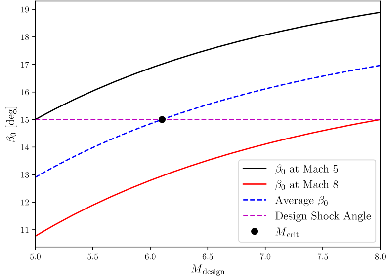
Fig. 3. Shock angle at symmetry plane against M_{\text{design}} .
