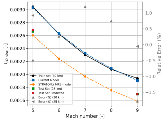
Fig. A.15. Viscous correction evaluation for waverider number 67.
