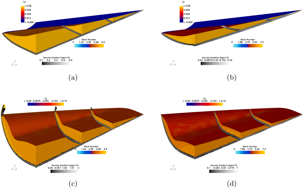
Fig. 11. Flow field contours of Mach number and density gradient as well as surface pressure coefficient: geometry 67 at (a) Mach 5, 25 km, and (b) Mach 8, 30 km; geometry 42 at (c) Mach 5, 25 km, and (d) Mach 8, 30 km condition. The same focal point is applied for these visualisations. Three axial cuts are shown with flow going from right to left.
