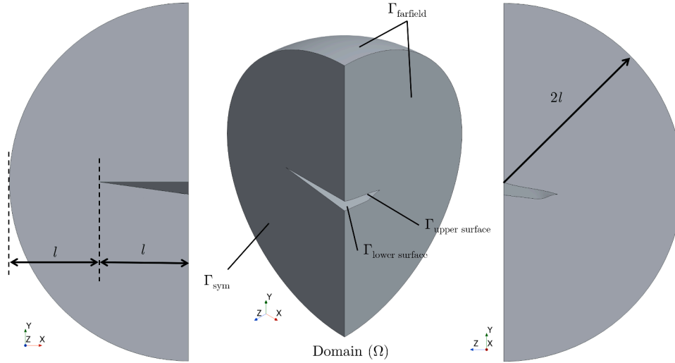
Fig. 6. Inviscid domain \Omega \in \mathbb{R}^3 used in this study, showing a view from the symmetry plane (left), isometric view (middle) and view from the back plane (right).
