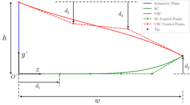
Fig. 2. Parametrisation of the base plane.
