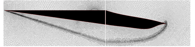
Fig. 7. AMR on the symmetry plane (left) and back plane (right) with n_{\text{ref}} = 3 .
