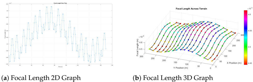
Figure 2. (a) Two dimensional (2D) and (b) 3D visualisations of how the focal length (zoom) changes at each waypoint during flight over Terrain Type 2. The UAV maintains a fixed altitude while adjusting zoom to preserve GSD.
