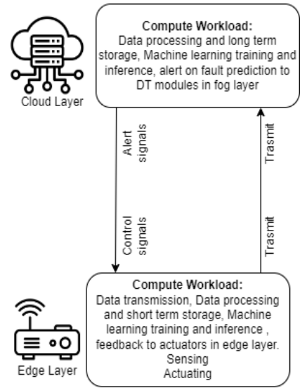
Figure 7: Architecture for Scenario B
