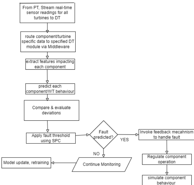
Figure 2: Predictive Digital Twin Workflow with Feedback
