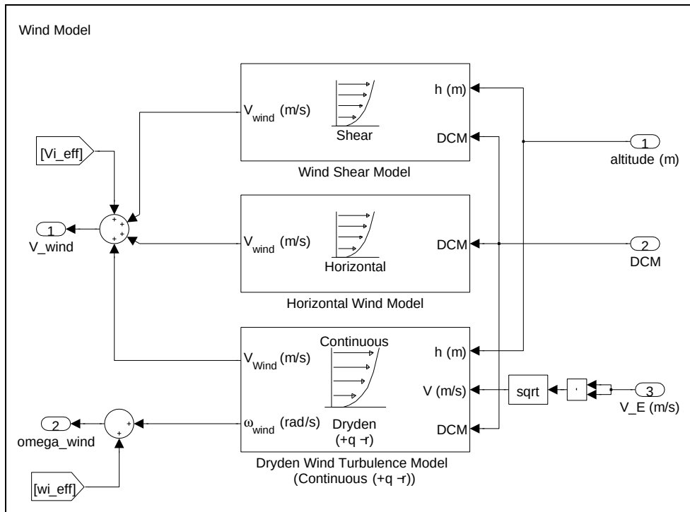
Figure 10: UAV Wind Model
