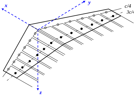
Figure 2: Modelling of the wing
