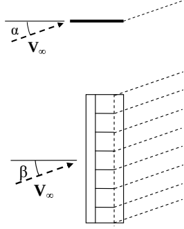
Figure 1: Vortex sheet positioning
