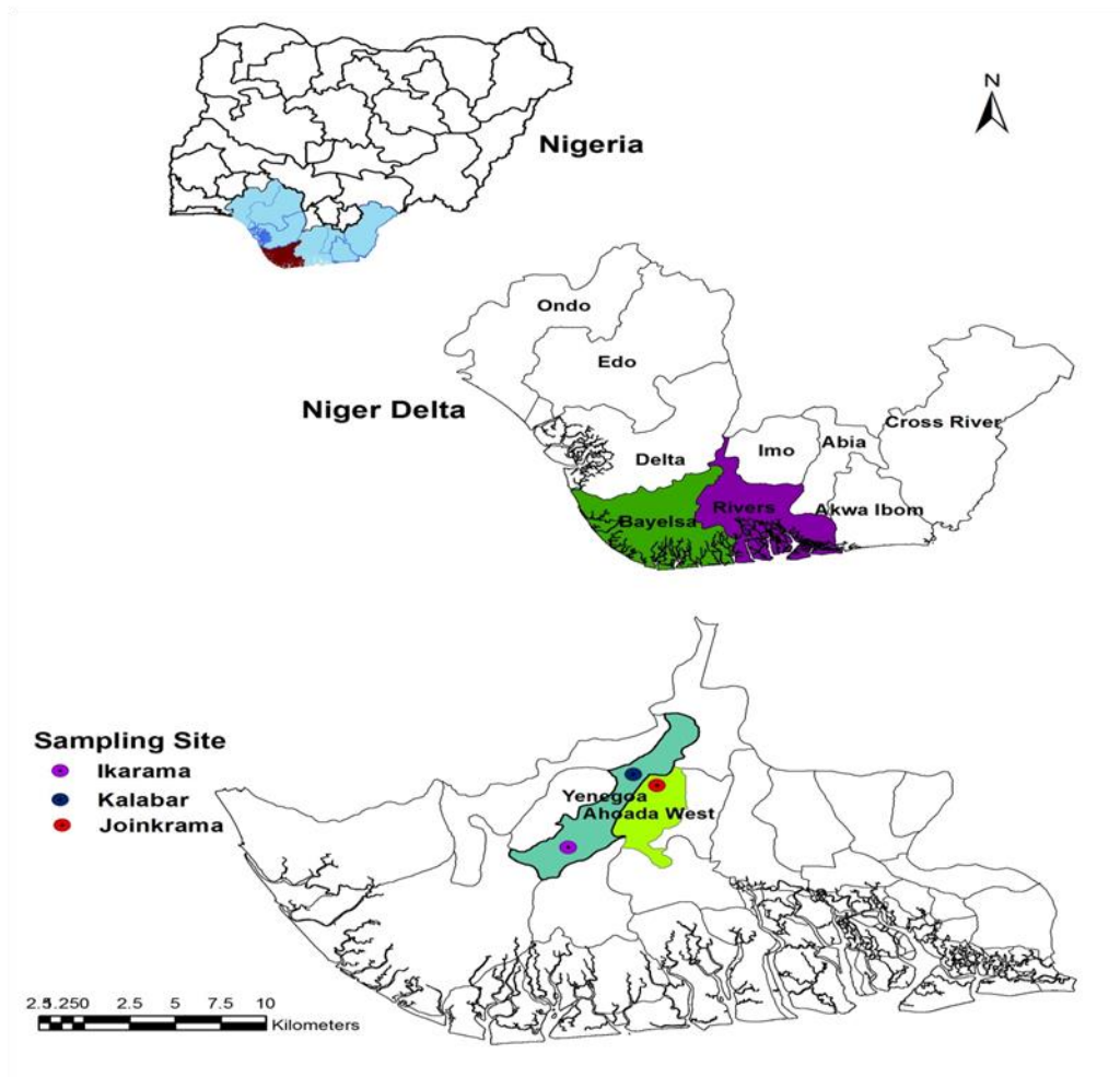
Figure 1 Soil sampling locations for the three contaminated sites in the Niger Delta (Bayelsa and Rivers State), Nigeria (After: Douglas et al., 2018).
