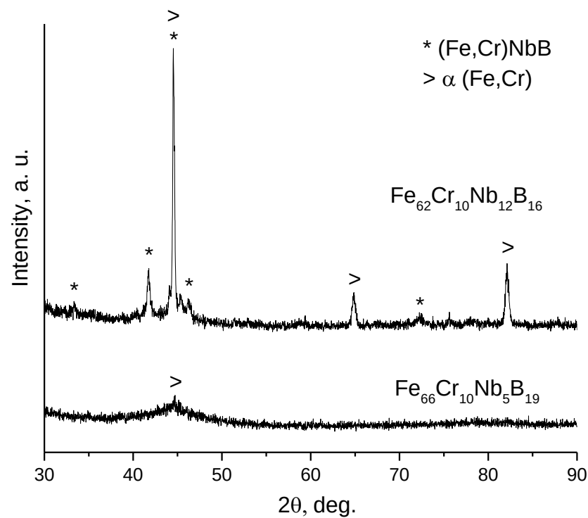
Figure 3. XRD patterns of the glassy \text{Fe}_{66}\text{Cr}_{10}\text{Nb}_5\text{B}_{19} alloy and crystalline \text{Fe}_{62}\text{Cr}_{10}\text{Nb}_{12}\text{B}_{16} alloy powders. (Fe,Cr)NbB has a hexagonal structure (space group P\bar{6}2m ).
