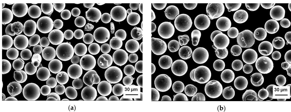
Figure 2. Morphology of the Fe-based alloy powders: (a) glassy Fe 66 Cr 10 Nb 5 B 19 and (b) crystalline Fe 62 Cr 10 Nb 12 B 16 (20–40 µm fraction).
