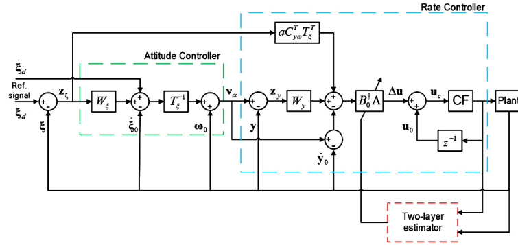
Fig. 1. Controller structure.
