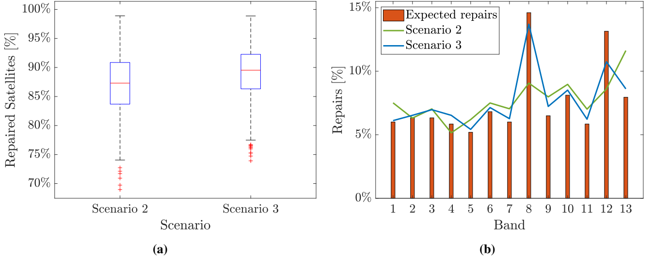
Fig. 9 Repaired satellite of Scenario 2 and Scenario 3 results. In Figure 6a the percentage of failed satellites repaired by the spacecraft and in Figure 6b the band's relative performance compared to the assigned satellite per band.
