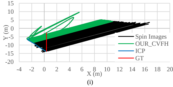
Fig. 4. 2D odometry plots for the SLA scenario (a)-(h) proposed architecture under various configurations, (i)-(j) competitor odometry methods
