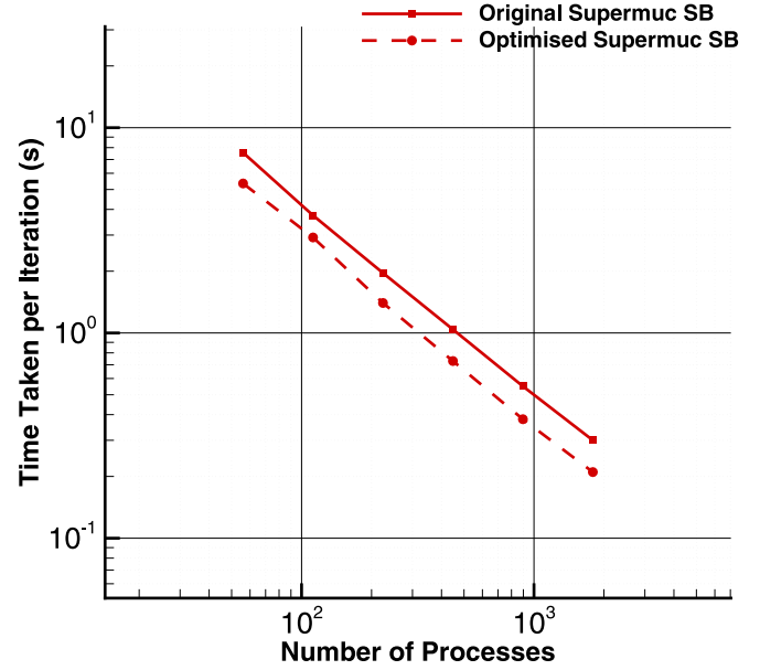
Fig. 8. Strong scalability results for the ILES of the Taylor–Green vortex using the WENO 2nd-order scheme on the finest tetrahedral mesh.
