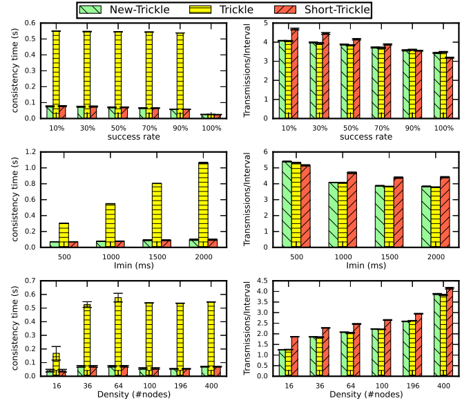
Fig. 3. Performance evaluation in single-hop networks
