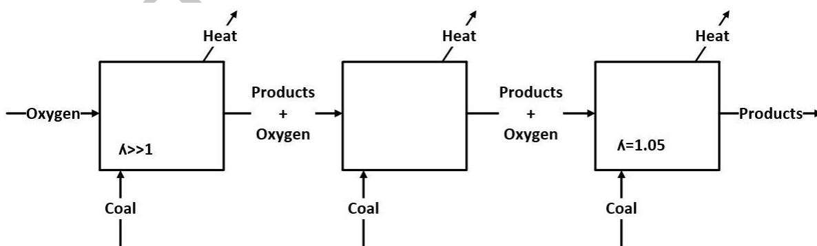
Figure 1. Depiction of staged pressurised oxy-combustion concept [16]
