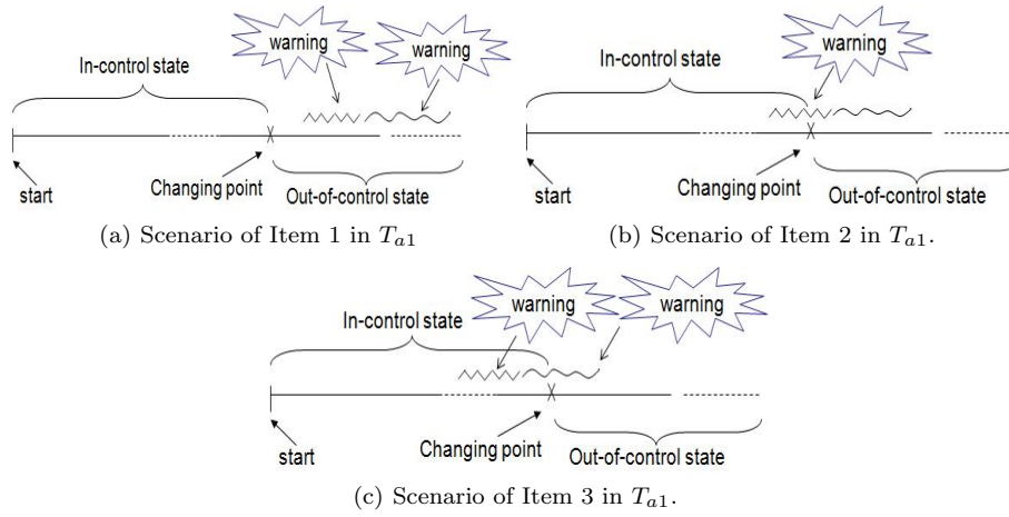
Fig. 3 Three scenarios in E(T_{a1}) (where the zigzag lines represent a sampling with the normal sample size n_0 and the wave lines represent a sampling with the larger sample size n_1 )
