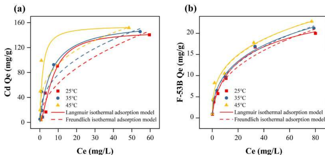
Figure. 4 Sorption isotherms of individual (a) Cd(II) and (b) F-53B by MMT/S-nZVI at 25, 35 and 45°C.
