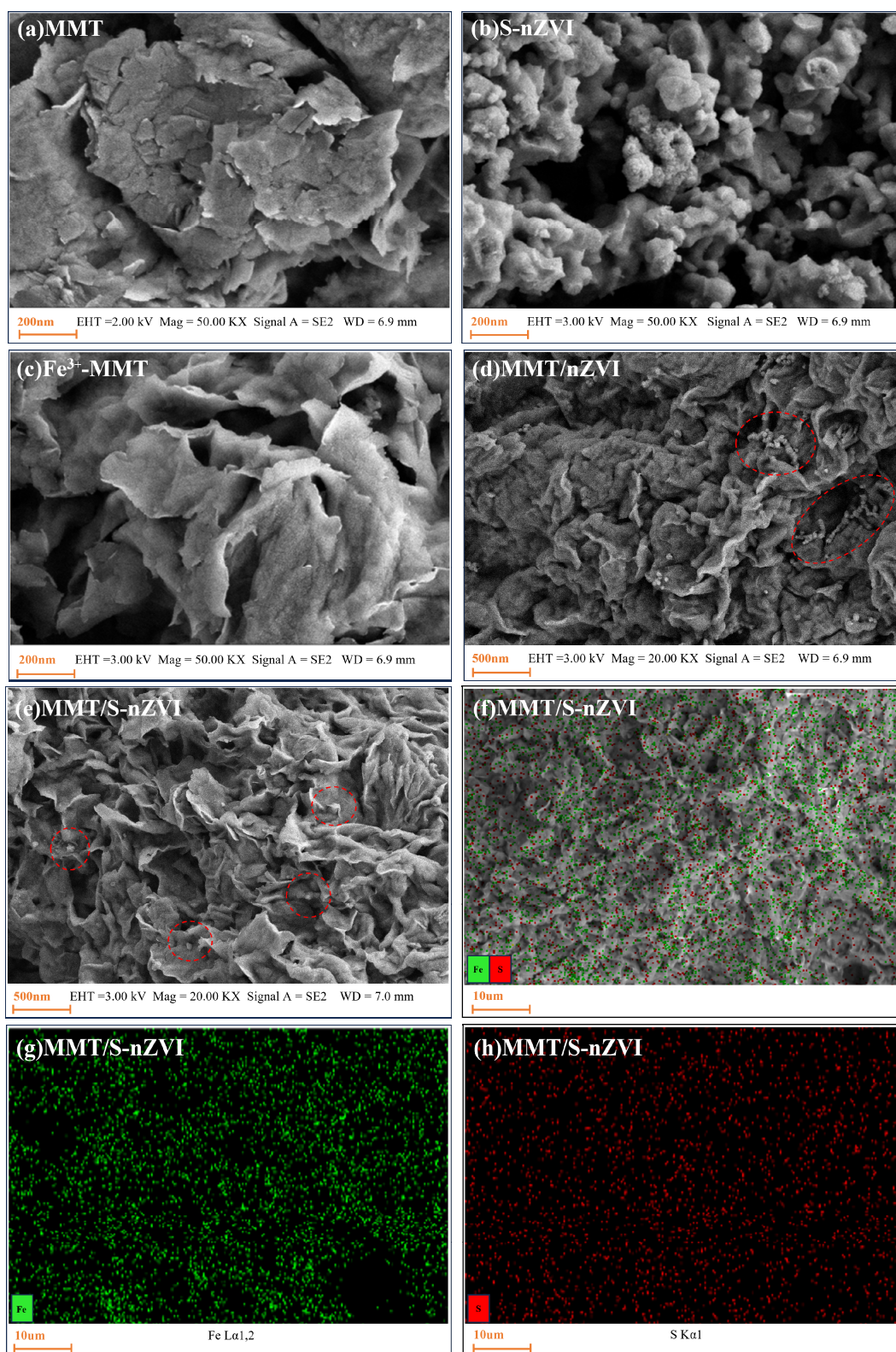
Figure 1 Morphology of (a) MMT, (b) S-nZVI, (c) \text{Fe}^{3+} -MMT, (d) MMT/nZVI, (e) MMT/S-nZVI obtained from SEM, and (f-h) EDS diagrams of MMT/S-nZVI.
