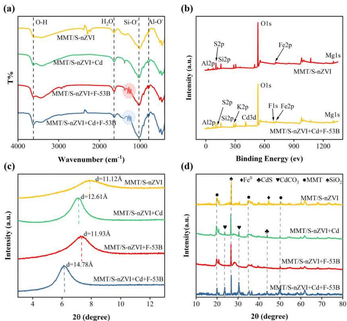
Figure. 7 Characterization of MMT/S-nZVI before and after reaction: (a) FTIR spectra; (b) XPS spectra of full spectrum scan; XRD spectra of 2θ range from (c) 3° to 12° and (d) 10° to 80°.
