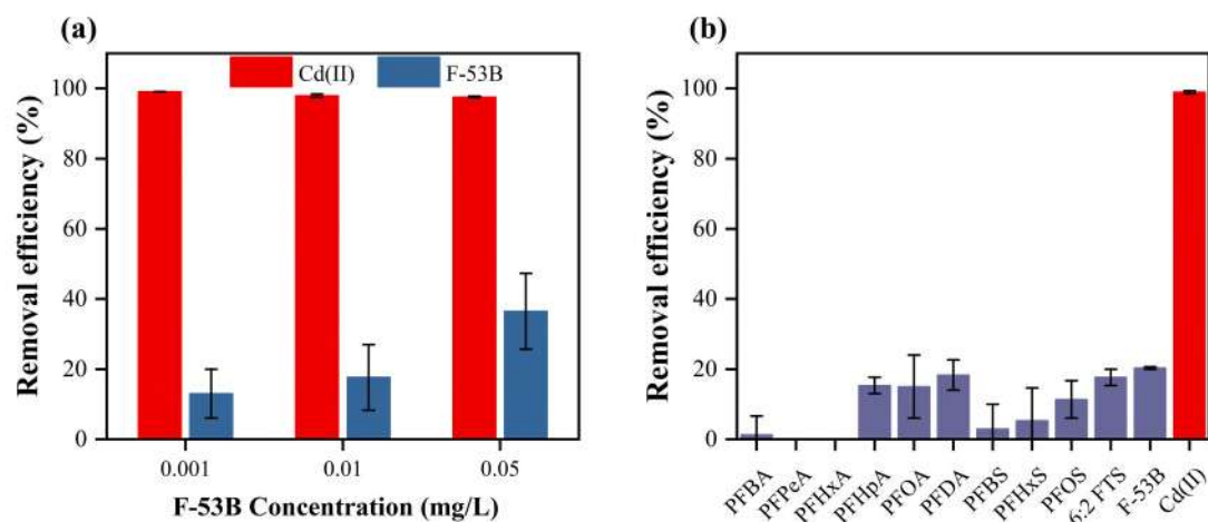
Figure. 6 Removal efficiency of Cd(II) and F-53B co-contamination (a), Cd(II) and the mixture of 11 PFASs (b) by MMT/S-nZVI at environmentally relevant levels. The concentrations were 0.2 mg/L for Cd(II) and 0.001 mg/L for each PFAS compound.
