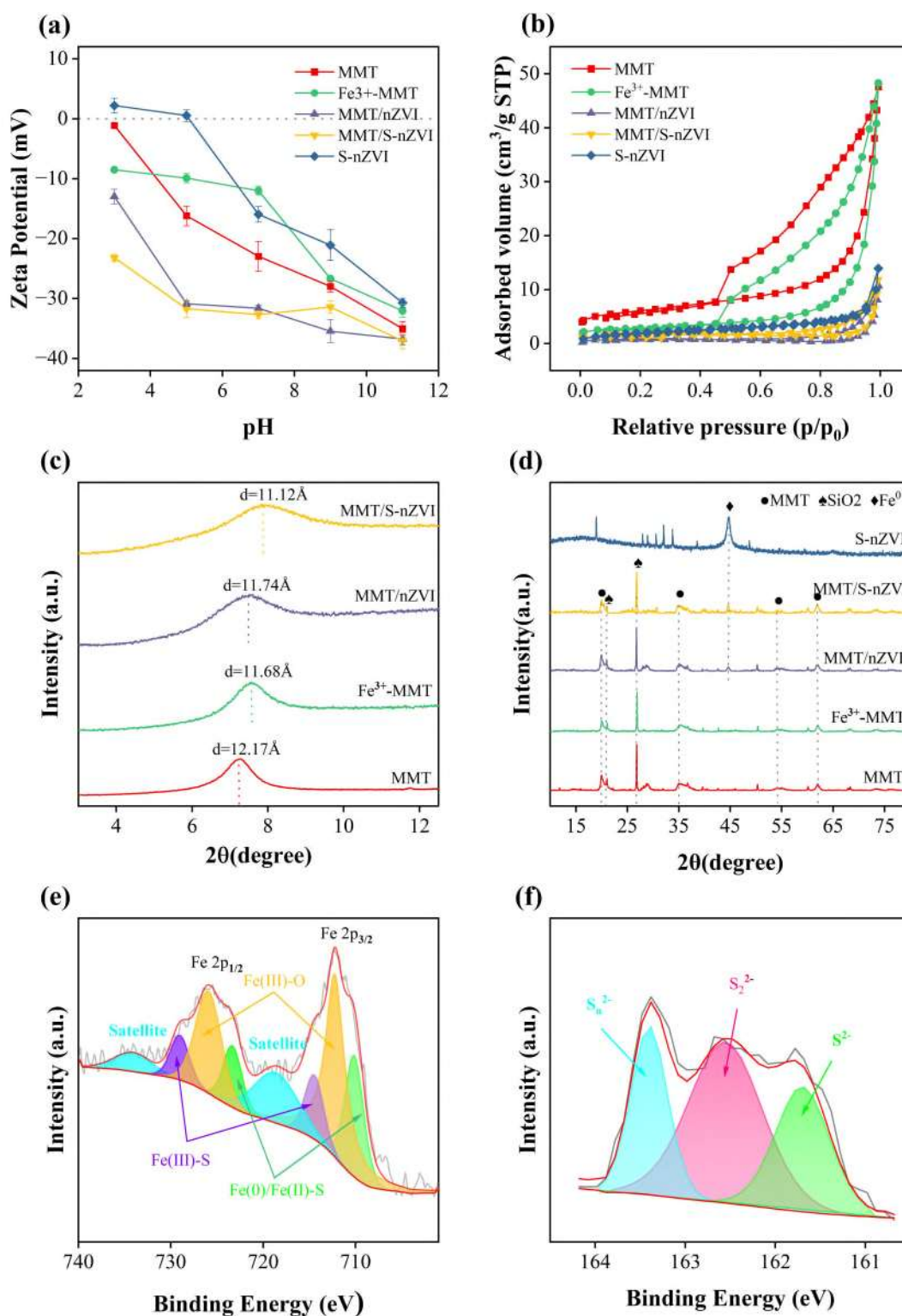
310 Figure. 2 (a) Zeta potential of materials; (b) N 2 adsorption-desorption isotherms of 311 materials; XRD patterns of materials within 2θ range of (c) 3°-12° and (d) 10°-80°; (e) 312 Fe 2p and (f) S 2p XPS spectrum of MMT/S-nZVI.
