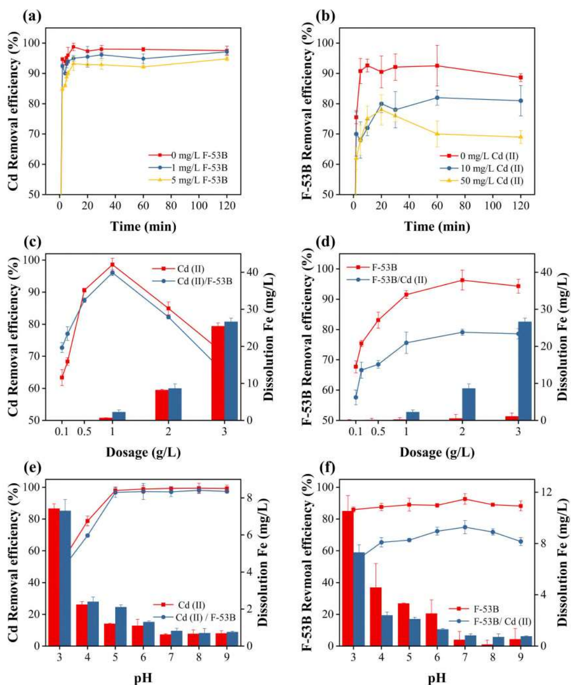
Figure. 5 Effects of experimental parameters on the removal of Cd(II) and F-53B by MMT/S-nZVI: (a, b) influence of initial contaminant concentrations; (c, d) effect of MMT/S-nZVI dosage on removal efficiency and Fe ion concentration; (e, f) impact of initial solution pH on removal efficiency and Fe ion release. Removal efficiencies are shown as line graphs, and Fe ion concentrations as bar graphs. Initial concentrations of Cd(II) and F-53B were 50.0 mg/L and 1.0 mg/L, respectively..
