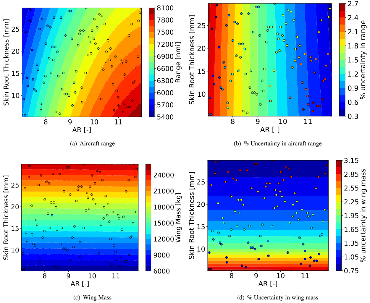
Fig. 5 2D Kriging surrogate model results using initial data provided by the user and % uncertainty obtained for the 2D design space; AR - aspect ratio
