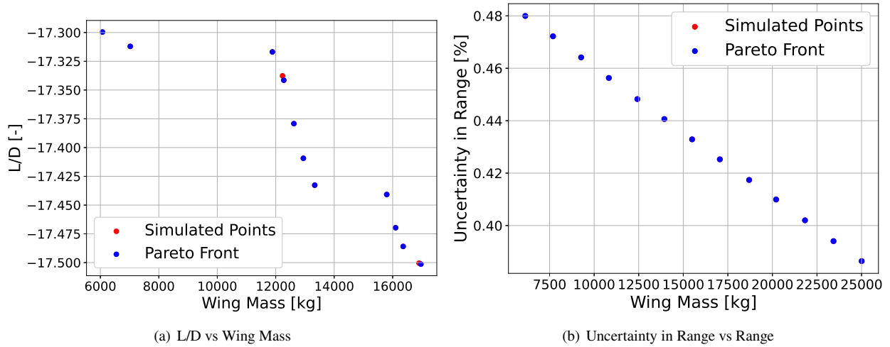
Fig. 7 Results for multi-objective optimisation showing Pareto fronts and design trade-offs for a robust design
