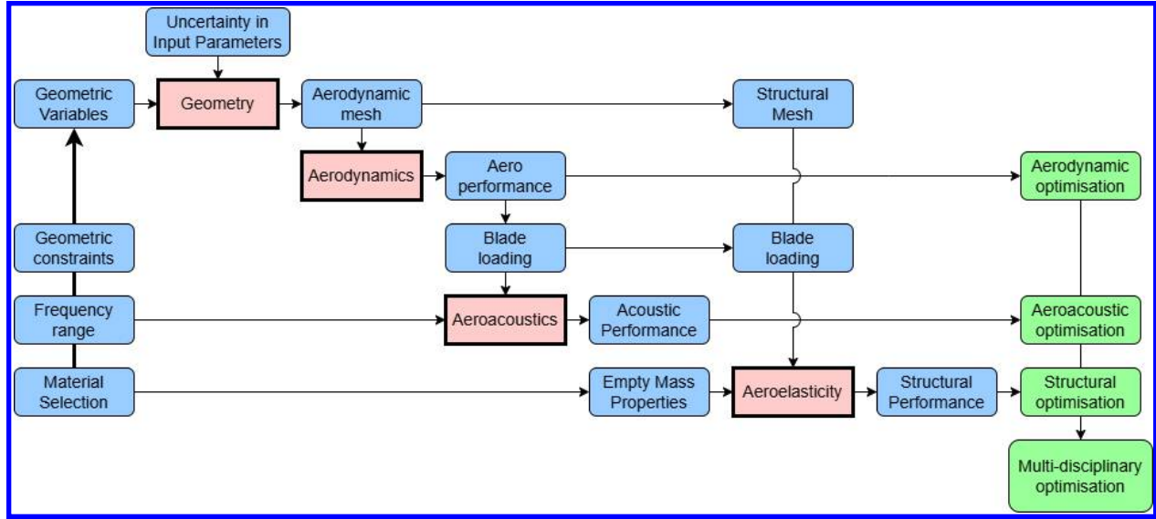
Fig. 1 System-level overview of the proposed Multi-Fidelity Multi-Disciplinary Optimisation (MFMDO) workflow for generating initial data for Visual Analytics
