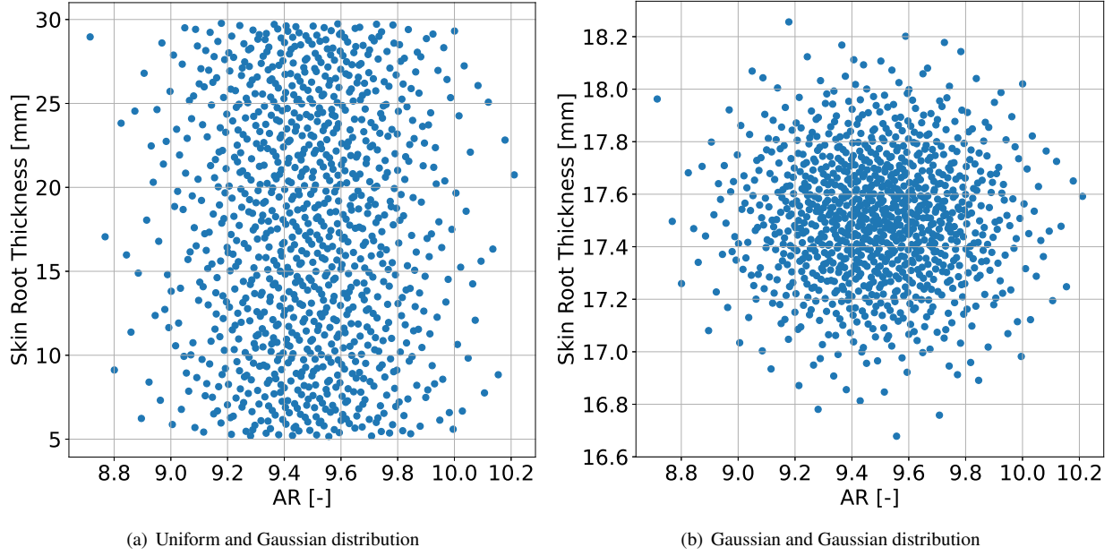
Fig. 6 Different types of sampling distribution for uncertainty quantification using the Halton sequence
