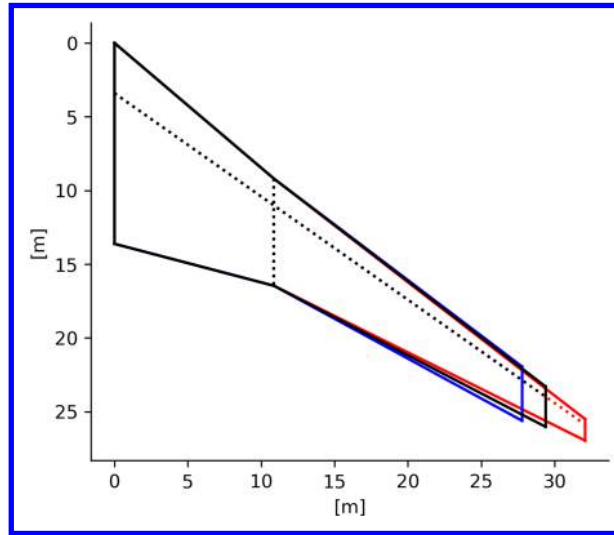
Fig. 3 Top view of the baseline CRM wing, with the two modifications highlighted in blue and red; adopted from Spinelli et al.
