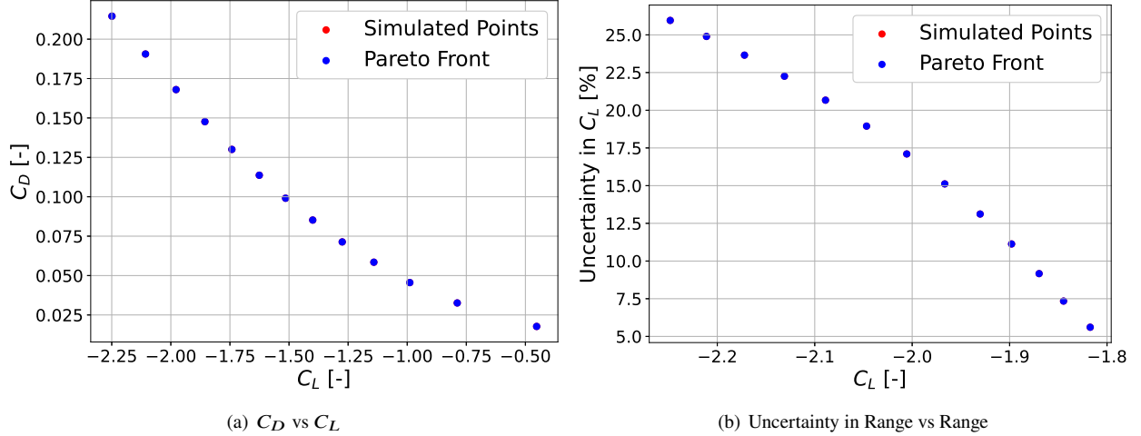
Fig. 9 Results for multi-objective optimisation showing Pareto fronts and design trade-offs for a robust design
