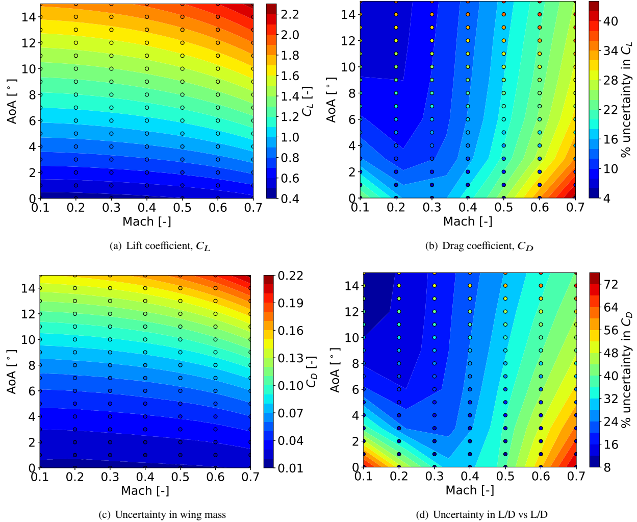
Fig. 8 2D Kriging surrogate model results for the ATI Narrowbody case study
