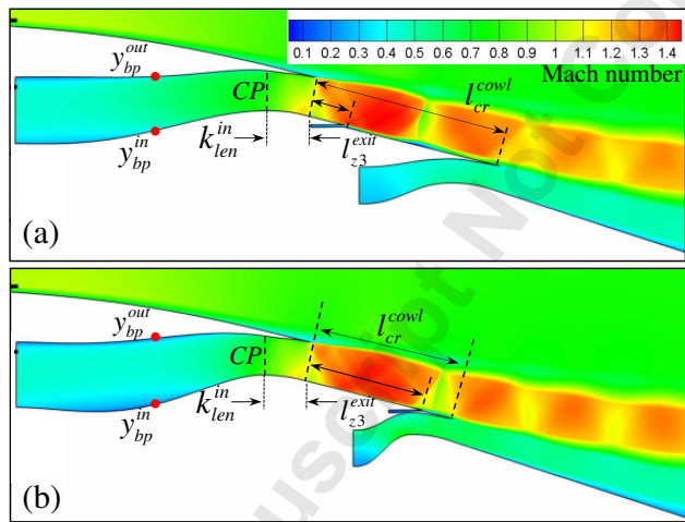
Fig. 13. Comparison between baseline and optimum exhaust designs for the current E2 engine architecture: (a) Baseline exhaust design, (b) Exhaust design optimized for C_V^{Overall}
