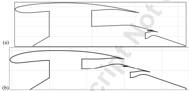
Fig. 5. 2D axis-symmetric geometries of investigated engine architectures: (a) Design representative of future engine architectures ( E1 ), (b) Design representative of current engine architectures ( E2 )
