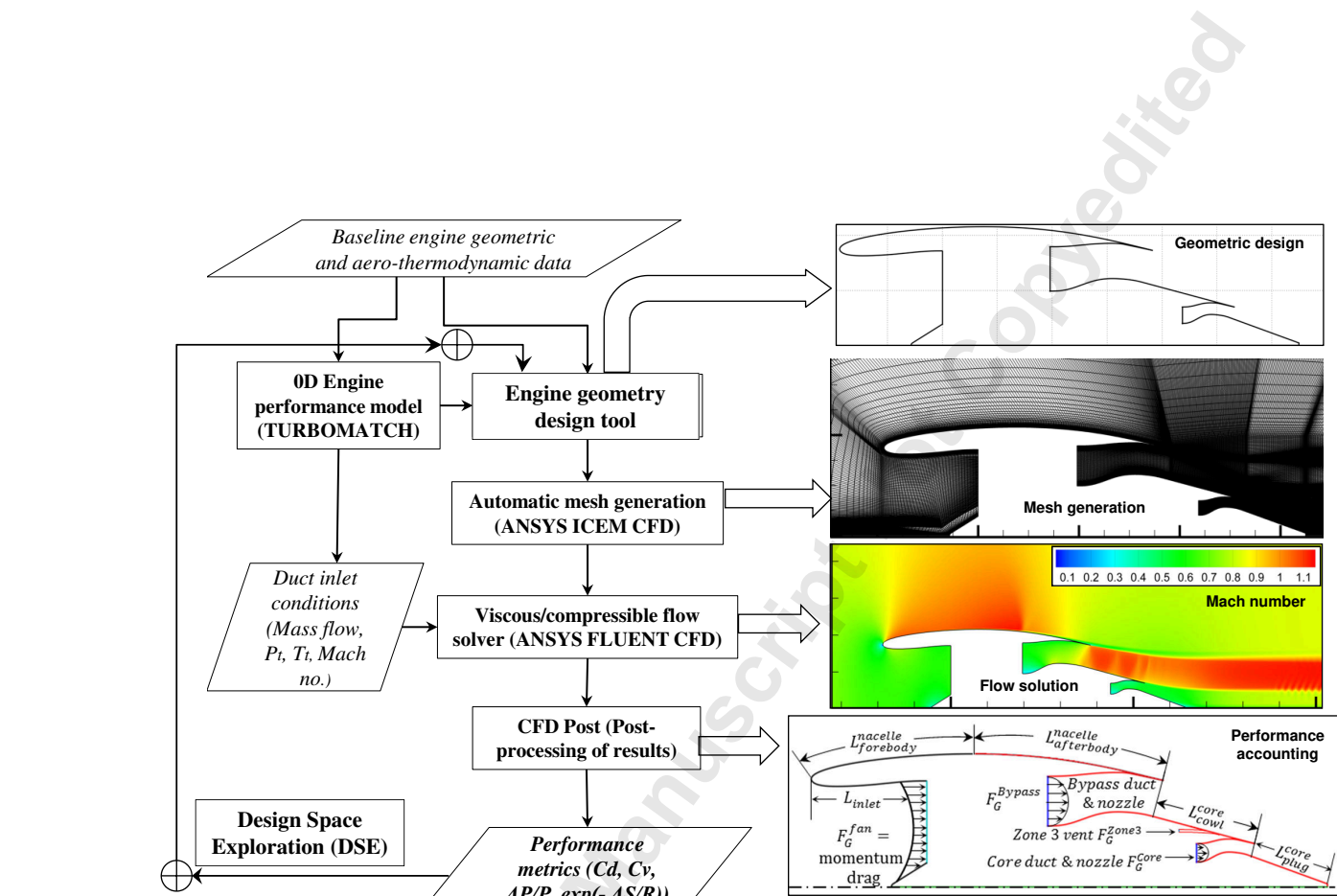
Fig. 2. Upper-level overview of the developed software architecture
