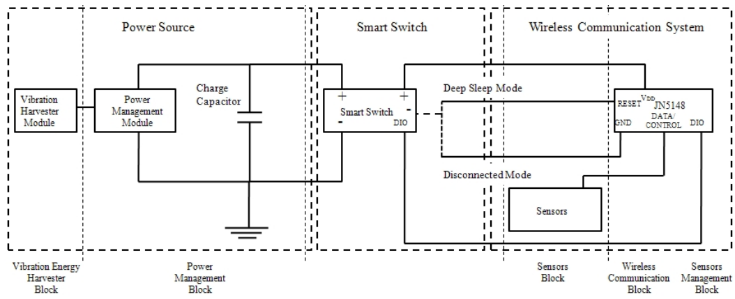
Fig. 1. System Design and Implementation at Hardware Level
