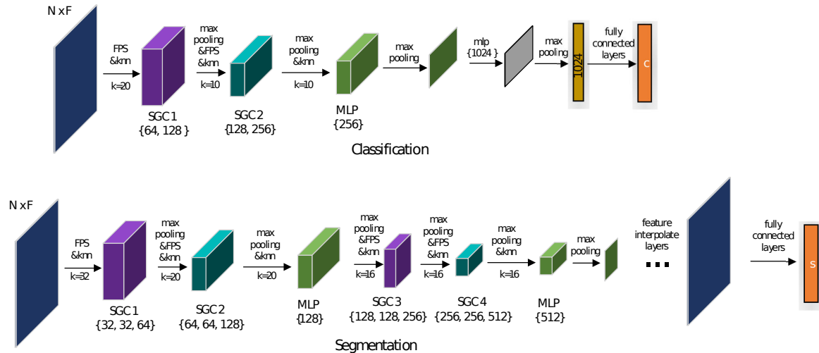
Figure 5. ShufflePointNet architecture: The architecture uses PointNet++ as backbone, and it contains classification structure (top branch) and semantic segmentation structure (bottom branch) for point cloud. In detail, N, F indicates the number of input points, and corresponding feature channels, respectively. k is the number of the neighbours. In addition, the number in the brace \{\} indicates the MLP filters. The classification model recursively applies Furthest Point Sampling (FPS) and a Shuffled Group Convolution (SGC) module to capture downsampled local features, followed by a shared full-connected layer to generate a global feature, which is used to predict classification scores. The segmentation model extends the classification model by two more SGC modules and a feature interpolation module to obtain a category score for each point.
