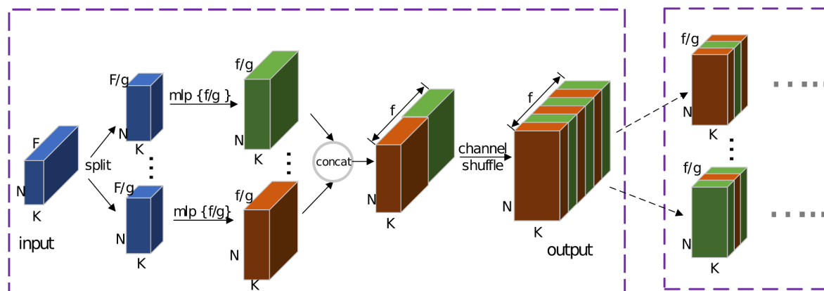
Figure 4. MLP Shuffled Group Convolution unit (SGC unit).
