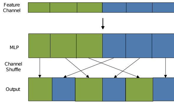
Figure 3. Ordered channel shuffle with MLP operation.
