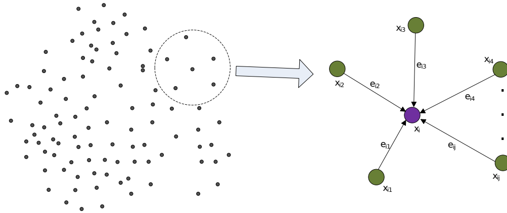
Figure 2. The process of construction of a directed acyclic graph for local feature extraction. On the left is the raw point cloud data, on the right, the graph-like structure extracted from part of the point cloud is represented. x_i indicates the central point, e_{ij} are the directed edges connecting center point and its corresponding neighbouring points x_{ij} .
