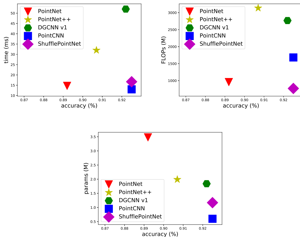
Figure 1. Measurement of accuracy, parameters, floating point operations (FLOPs) and forward time. It shows that our proposed ShufflePointNet (magenta diamond marker) tends to stay in the bottom-right corner, which means that our model conjugates high accuracy with low model complexity.
