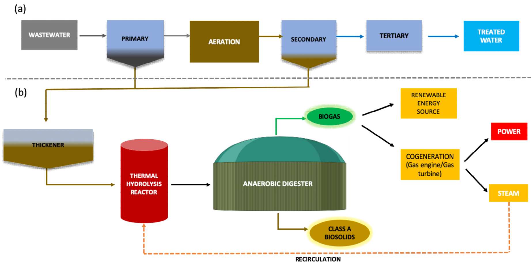
977 Fig. 1. Schematic representation of a wastewater treatment plant (WWTP) (a) without and (b) with thermal hydrolysis process (Ariunbaatar et 978 al., 2014)
