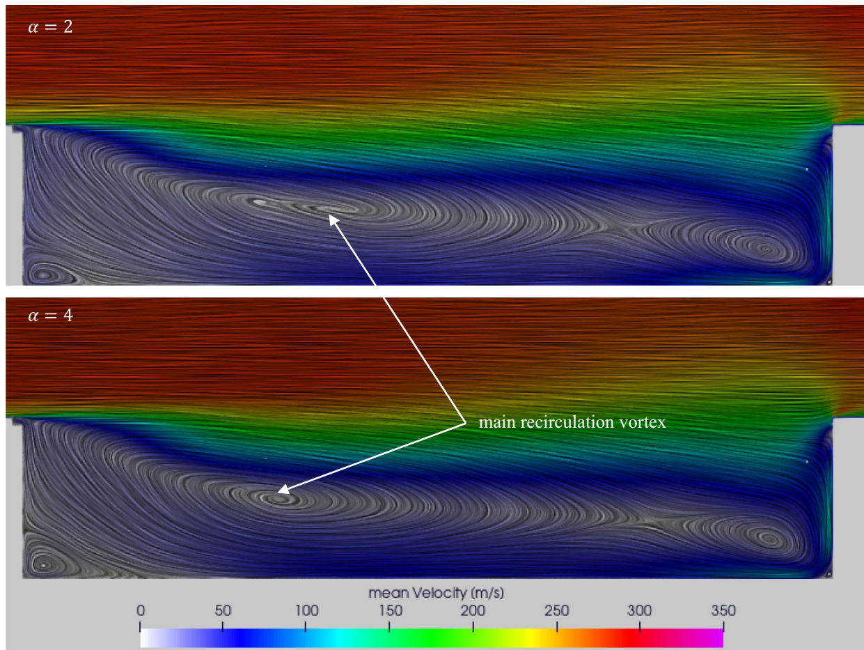
Fig. 10 LIC of mean flow velocity, coloured by velocity magnitude. Slice at 2y/W = 0 . Comparison of topology between \alpha = 2 (upper) and \alpha = 4 (lower). Mach 0.85. Flow from left to right
