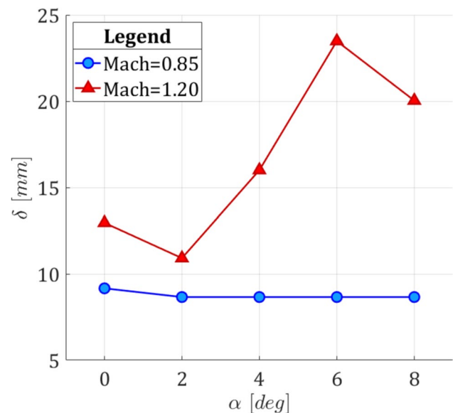
Fig. 9 Influence of angle of attack on the boundary layer thickness at the cavity leading edge
