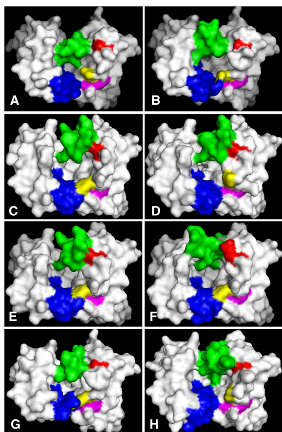
Fig. 2 The effect of amino acids within CDR H2 on the predicted positioning of CDRs H3 and L3. Amino acid positions H53 (red), H58 (yellow), and H59 (magenta) in clones a HSL1, b HSL2, c SQA A5, d SQA B3, e POR B11, f POR A7, g COP H3, and h COP A8. Position H53 has a profound effect on the orientation of CDR H3 (green), whilst positions H58 and H59 influence CDR L3 (blue) orientation. These homology images of the post-selection clones were constructed utilizing SWISS-MODEL workplace. The structures were viewed by PyMOL 1.3 (academic version)
