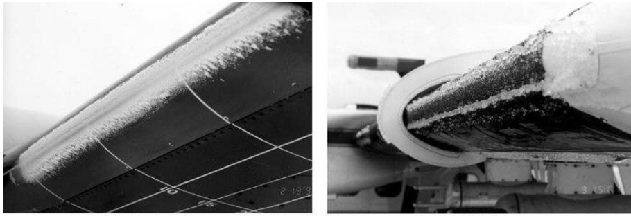
Figure 2.0-2 Comparison of rime ice (left), formed by small droplets freezing instantly, and glaze ice (right), formed by large droplets freezing slowly [20]
