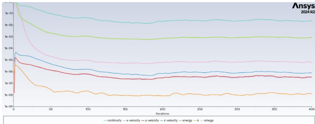
Figure C-9 Residual history for A320 cruise case
