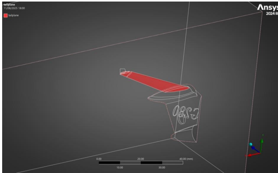
Figure 3.0-11 Tailplane faces of the Gulfstream G280 discretised with finer surface mesh.
