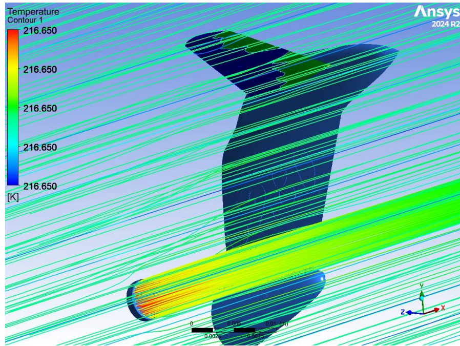
Figure 5-5 G280 cruise case: rear-mounted exhaust plume impinging on tailplane.
