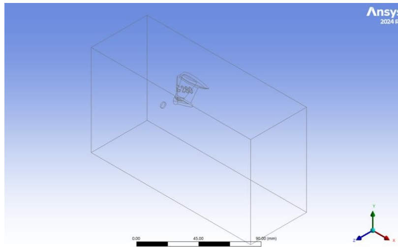
Figure 3.0-5 Computational domain of the Gulfstream G280 with rear-fuselage engines aligned with the tailplane.
