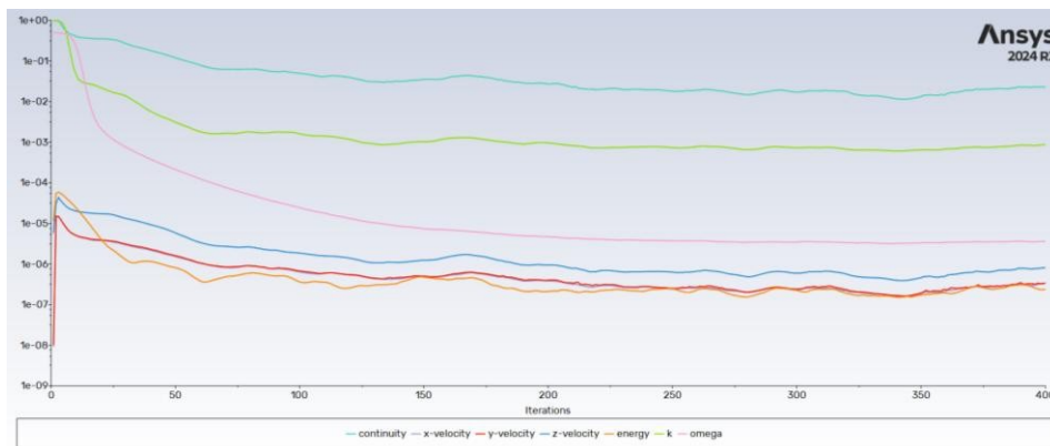
Figure 5-1 Residual history for the A320 cruise case, representative of the best residual convergence among all simulations
