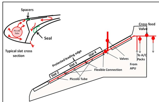
Figure 2.0-3 Pneumatic and electrothermal wing ice protection systems [22]
