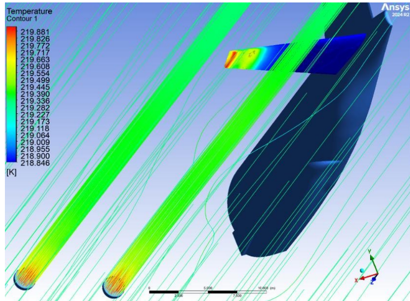
Figure 5-6 A380 cruise case: exhaust plume impinging on bottom surface of tailplane.
