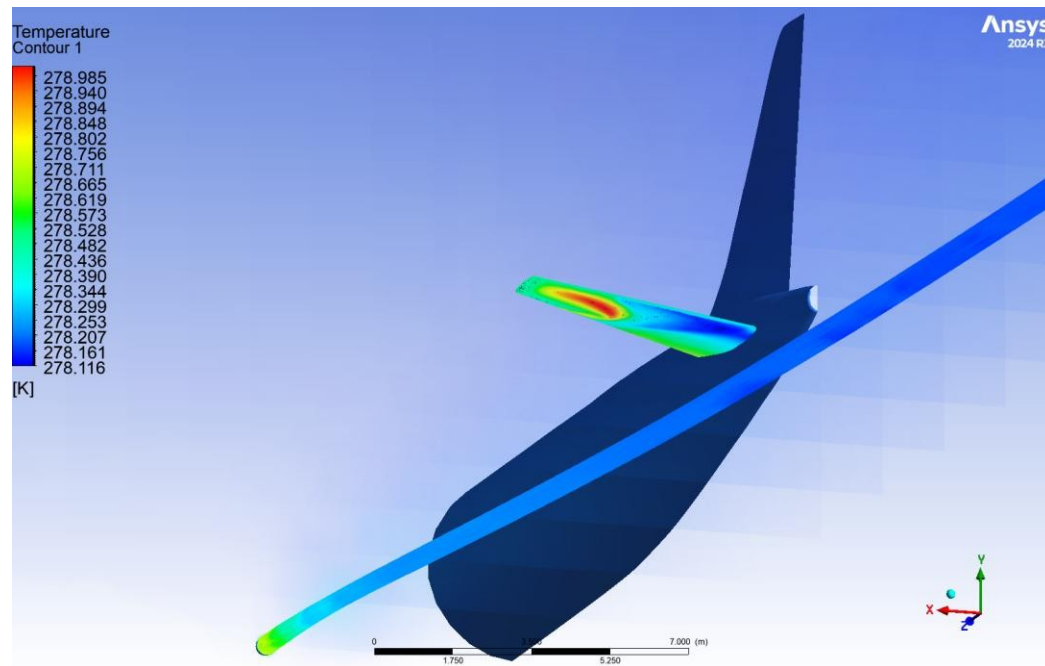
Figure D-10 A320 runway case: rear-mounted exhaust plumes and impinging on tailplane
