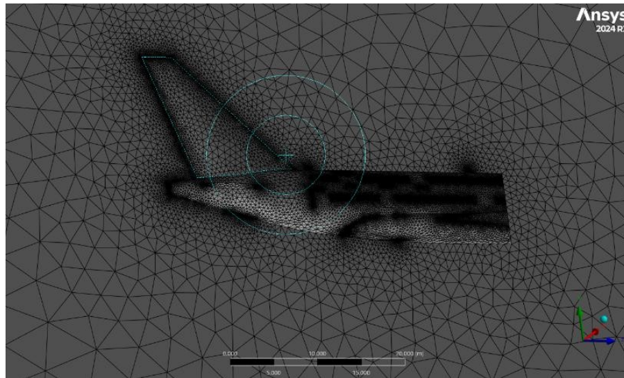
Figure 3.0-9 Overall mesh of the Airbus A380 computational domain viewed along the symmetry plane.
