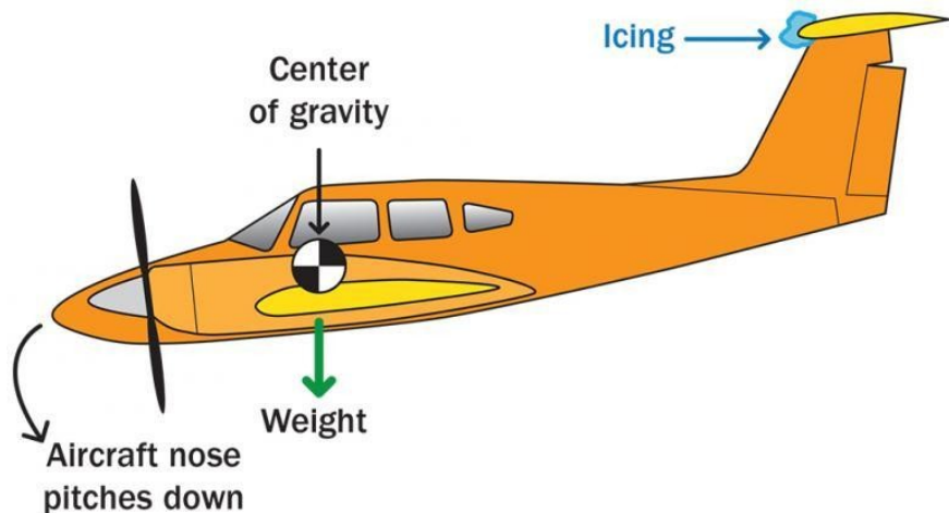
Figure 1.0-2 Effect of tailplane icing causing nose-down pitching moment [9]
