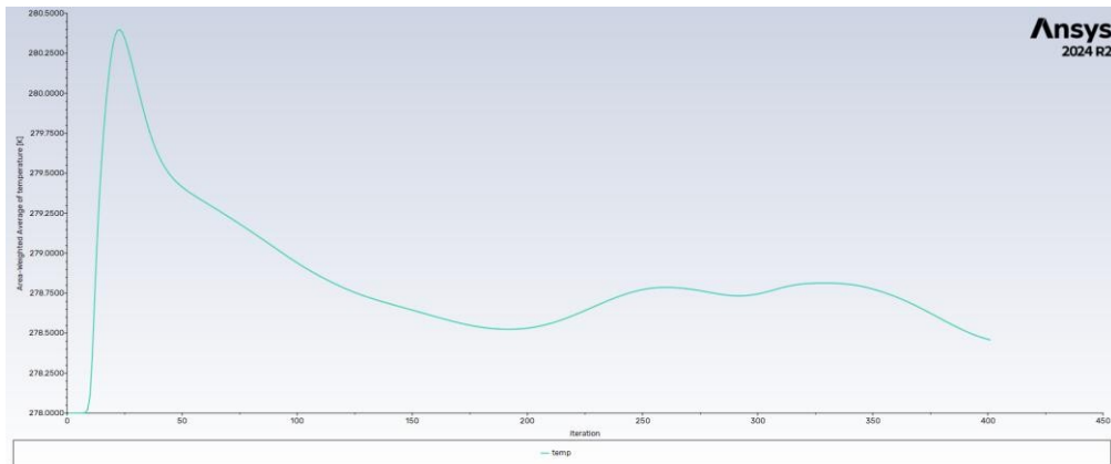
Figure C-8 Area-weighted average tailplane temperature for the A320 runway case
