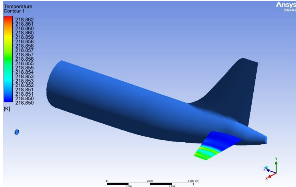
Figure D-1 Temperature contours of the A320 tailplane during cruise phase (upper rear angle view)
