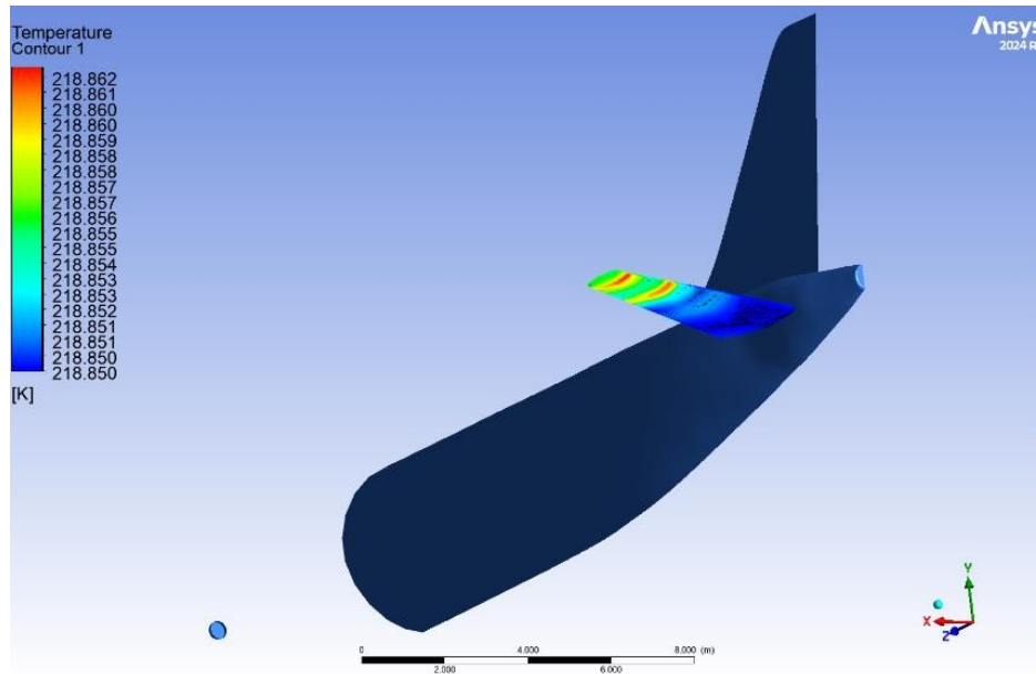
Figure D-2 Temperature contours of the A320 tailplane during cruise phase (low rear angle view)
