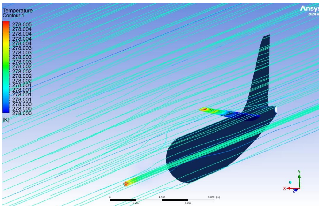
Figure D-8 Inlet streamlines superimposed with temperature contours during taxiing phase(20kts headwind)
