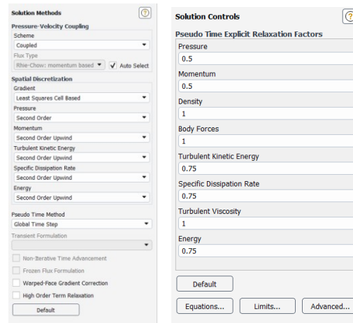
Figure 4.0-1 Solution Method(left) and Solution Controls(right) for all solved variables
