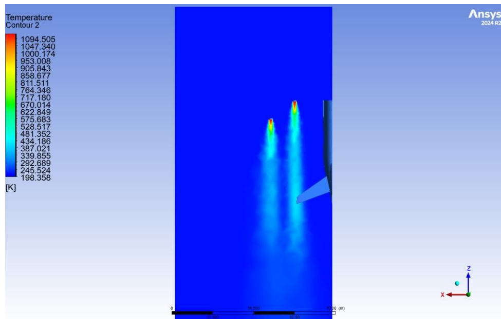
Figure E-3 Temperature contour of exhaust gases during A380 cruise phase (top view)
