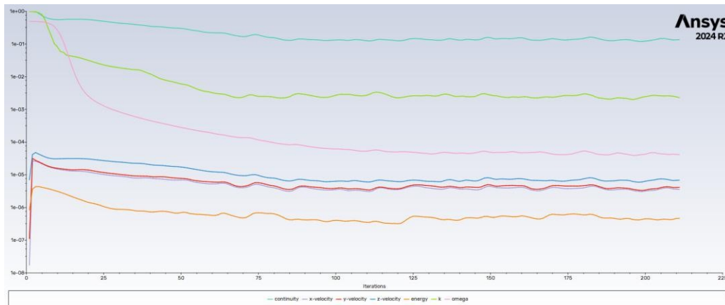
Figure 5-3 Residual history for A320 take-off case
