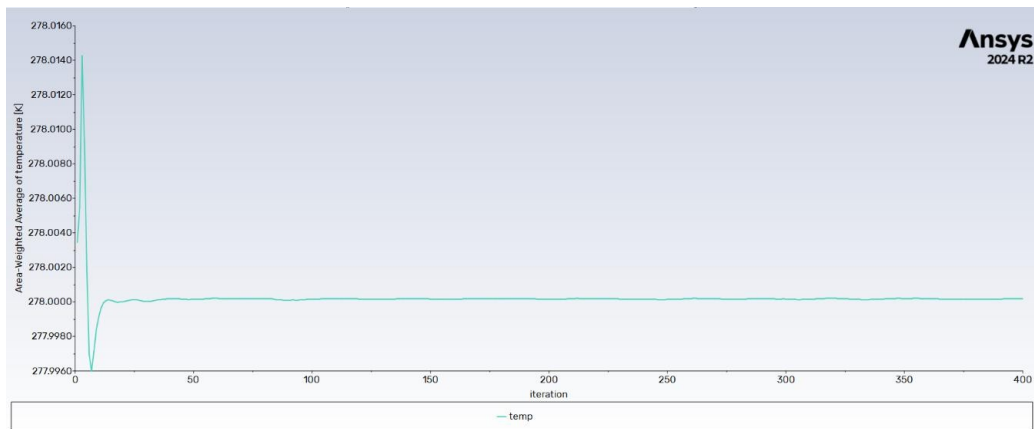
Figure C-10 Area-weighted average tailplane temperature for the A320 cruise case
