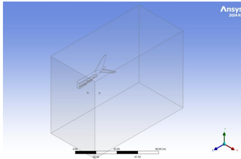
Figure 3.0-6 Computational domain of the Airbus A380 with large underwing engines and extended enclosure.
