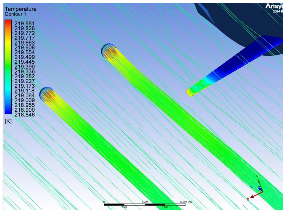
Figure D-6 A380 cruise case: rear-mounted exhaust plume impinging on tailplane (upper rear angle view)
