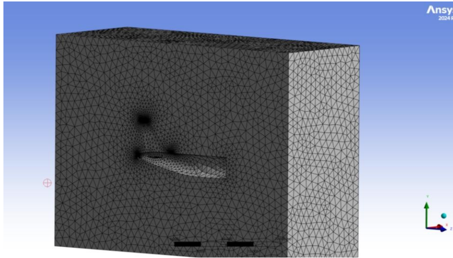
Figure 3.0-7 Overall mesh of the Airbus A320 computational domain viewed along the symmetry plane.
