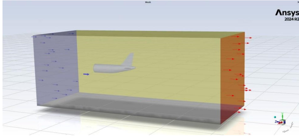
Figure 3.0-13 Computational domain in ANSYS Fluent showing the freestream inlet (blue), engine exhaust(single blue), pressure outlet (red) and aircraft geometry positioned within the enclosure. A symmetry plane is applied along the fuselage centreline to halve the domain size.
