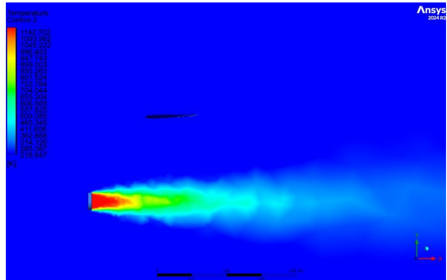
Figure E-2 Temperature contour of exhaust gases during G280 cruise phase (side view)
