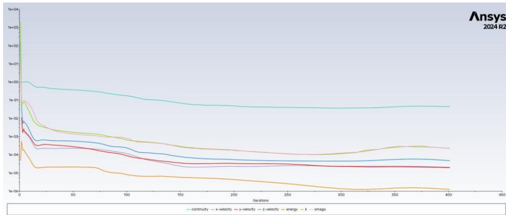
Figure C-7 Residual history for A320 runway case
