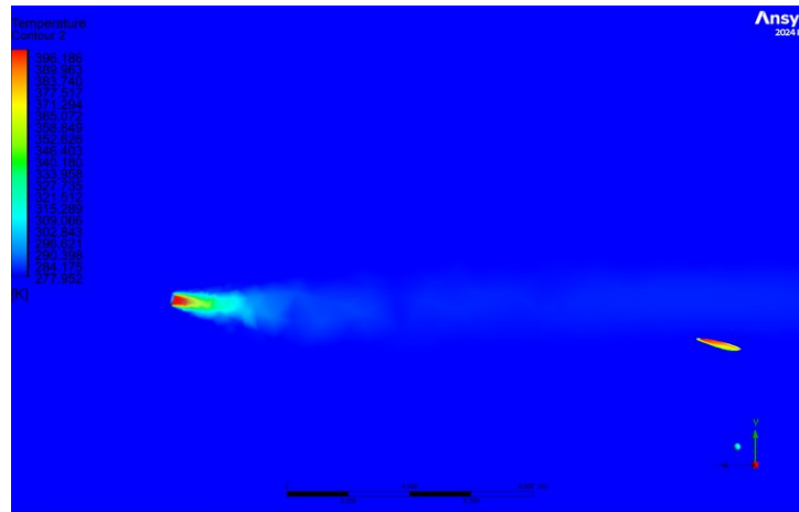
Figure 5-9 Temperature contour of exhaust gases during A320 take-off phase.
