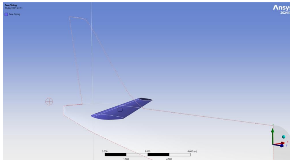
Figure 3.0-10 Tailplane faces of the Airbus A320 assigned finer mesh sizing for improved local resolution.
