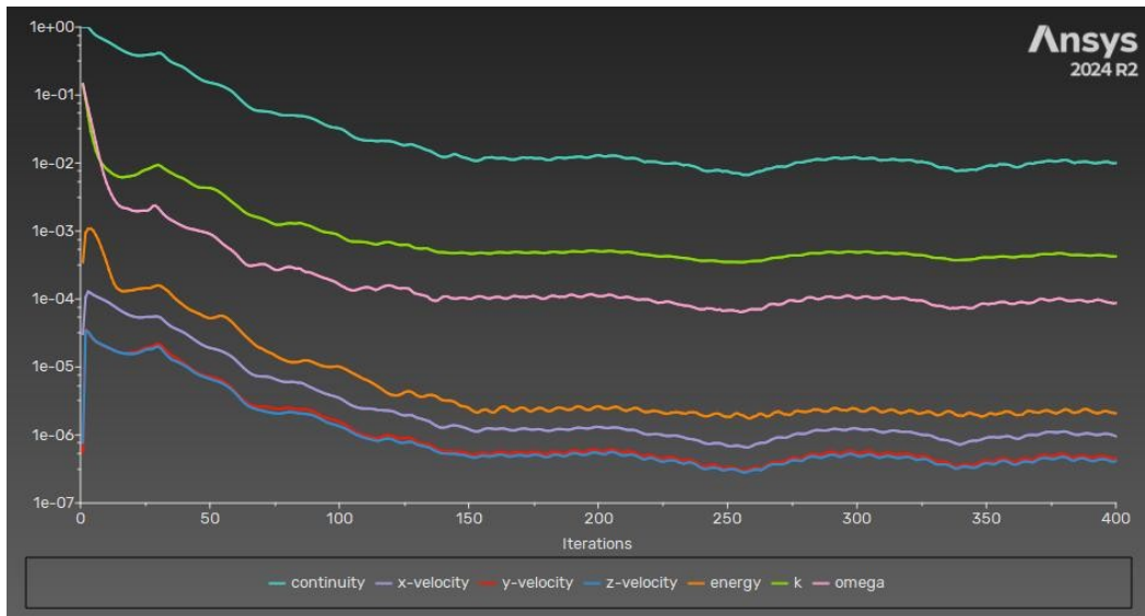
Figure C-2 Residual history for the G280 cruise case
