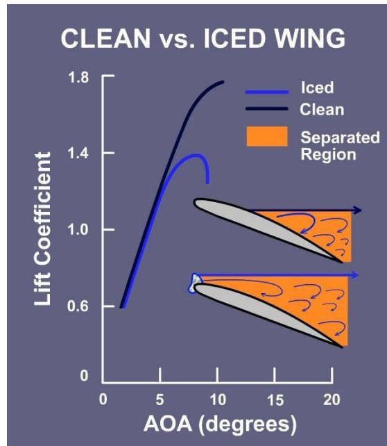
Figure 1.0-3 Lift reduction in clean wing vs iced wing [11]
