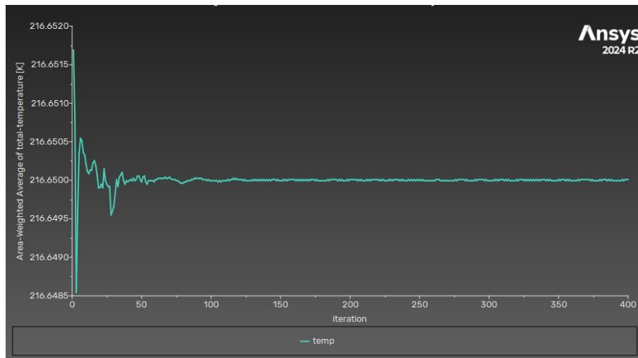
Figure 5-2 Area-weighted average tailplane temperature for the G280 cruise case, representative of the best thermal monitor across all cases
