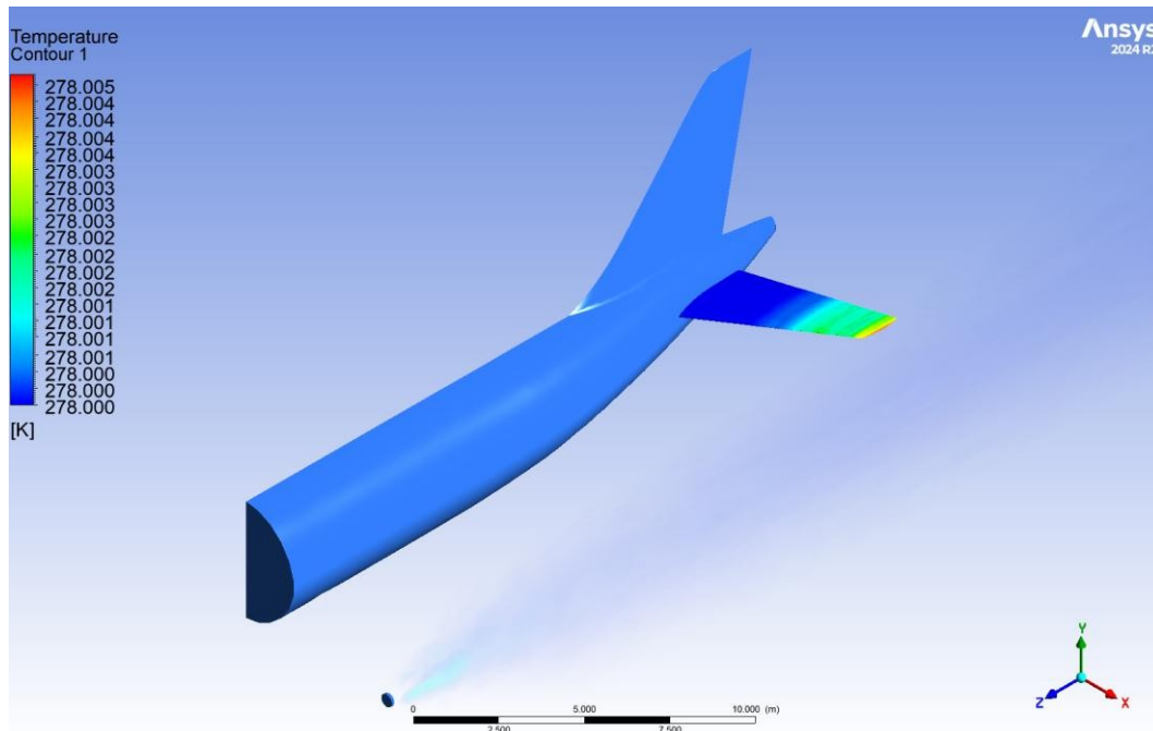
Figure D-7 Temperature contours of the A320 tailplane during taxiing phase
