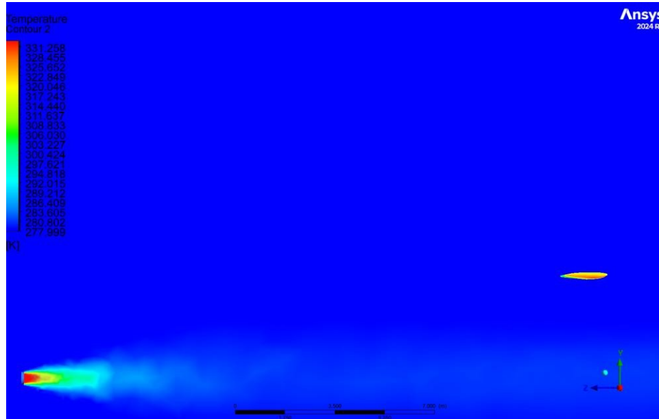
Figure E-4 Temperature contour of exhaust gases during A320 taxiing phase
