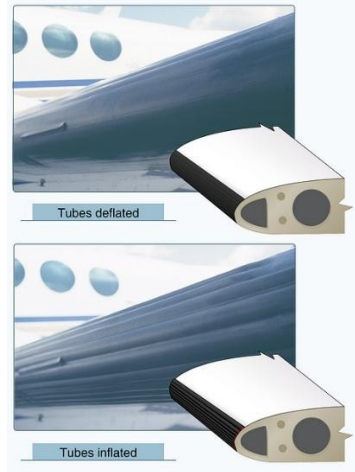
Figure 2.0-2 Deflated and inflated deicing boots on the LE of the wing [23]
