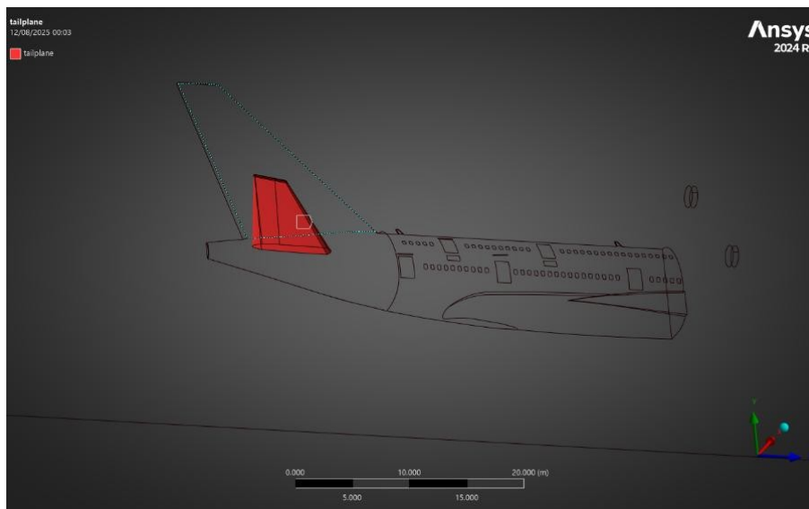
Figure 3.0-12 Tailplane faces of the Airbus A380 meshed with local refinement to capture heat transfer gradients.
