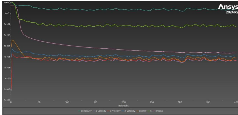
Figure C-3 Residual history for the A380 cruise case
