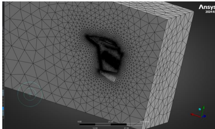
Figure 3.0-8 Overall mesh of the Gulfstream G280 computational domain viewed along the symmetry plane.
