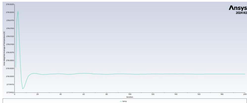
Figure C-6 Area-weighted average tailplane temperature for the A320 taxiing case
