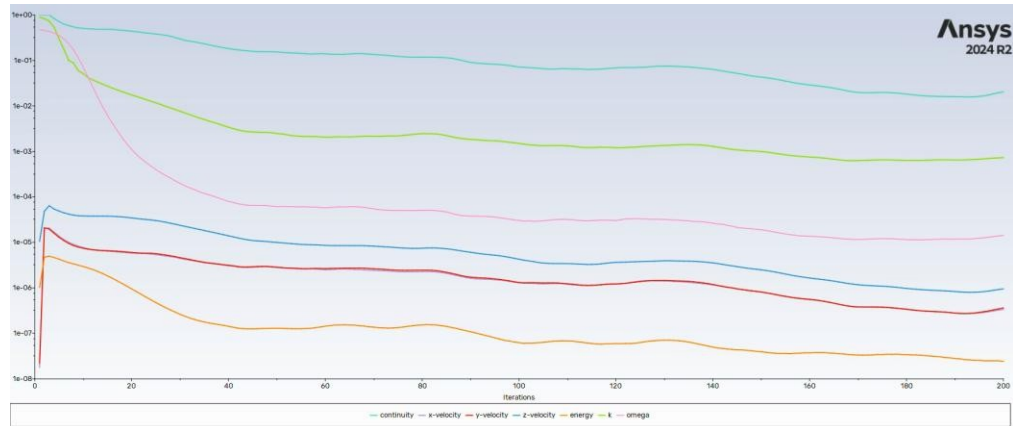
Figure C-5 Residual history for A320 taxiing case
