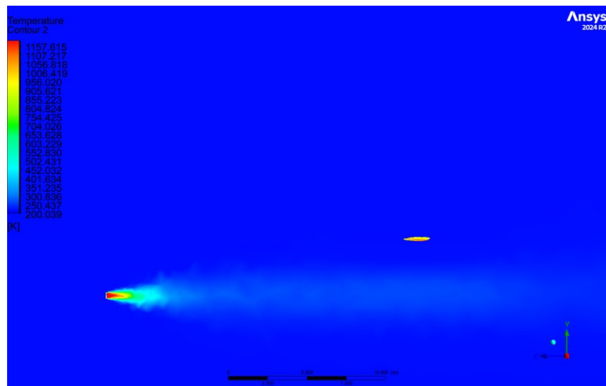
Figure E-1 Temperature contour of exhaust gases during A320 cruise phase (side view)
