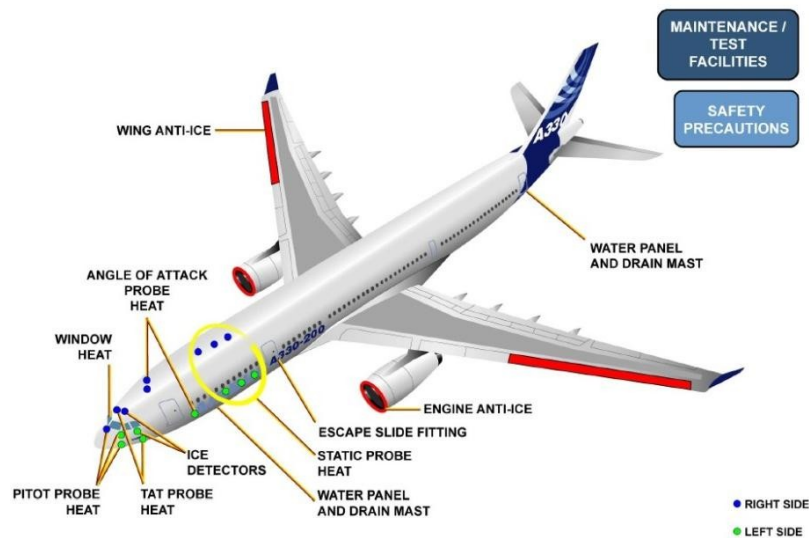
Figure 1.0-4 A330 ICE PROTECTION SYSTEM [15]
