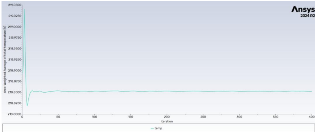
Figure C-1 Area-weighted average tailplane temperature for the A320 cruise case
