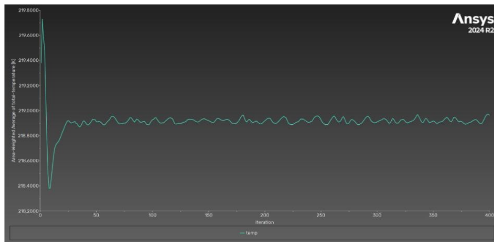
Figure C-4 Area-weighted average tailplane temperature for the A380 cruise case
