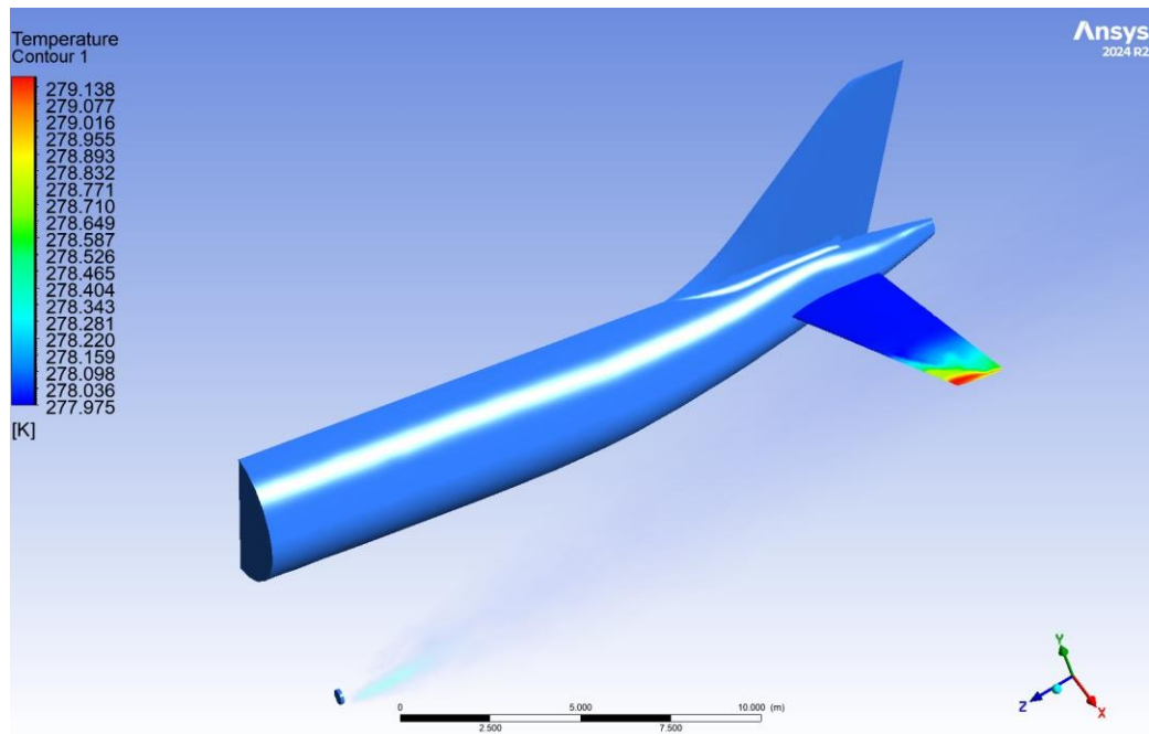
Figure D-11 Temperature contours of the A320 tailplane during take-off phase
