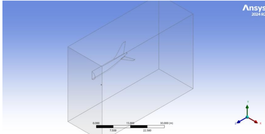
Figure 3.0-4 Computational domain of the Airbus A320 with underwing engines and symmetry applied.
