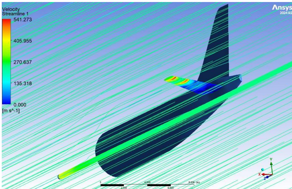
Figure D-3 A320 cruise case: rear-mounted exhaust plume impinging on tailplane
