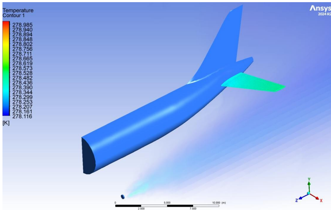
Figure D-9 Temperature contours of the A320 tailplane during runway phase
