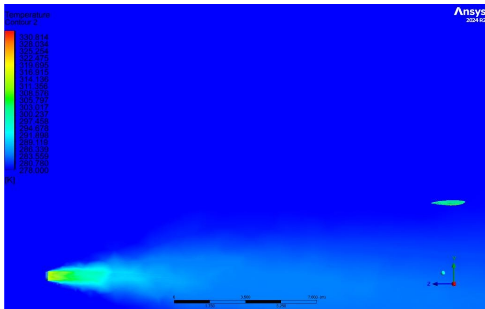
Figure E-5 Temperature contour of exhaust gases during A320 runway phase
