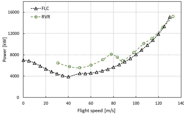
Figure 2: Total power requirement for compound rotorcraft as a function of flight speed at SL conditions
