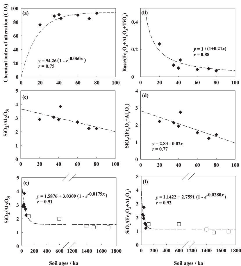
Figure 6 Weathering indices plotted against estimated soil age of Green Island profiles: (a) chemical index of alteration, \text{CIA} = \text{Al}_2\text{O}_3/(\text{Al}_2\text{O}_3 + \text{CaO} + \text{Na}_2\text{O} + \text{K}_2\text{O}) \times 100 , (b) base depletion = (\text{CaO} + \text{Na}_2\text{O} + \text{K}_2\text{O} + \text{MgO})/(\text{Fe}_2\text{O}_3 + \text{Al}_2\text{O}_3 + \text{TiO}_2) , (c and e) \text{SiO}_2/\text{Al}_2\text{O}_3 , (d and f) \text{SiO}_2/(\text{Fe}_2\text{O}_3 + \text{Al}_2\text{O}_3) ; time-scales in (e) and (f) are extended by combination with the data (open squares) of Zhang et al. (2007). The equation in each subfigure gives the prediction for relative soil ages by the given index.
