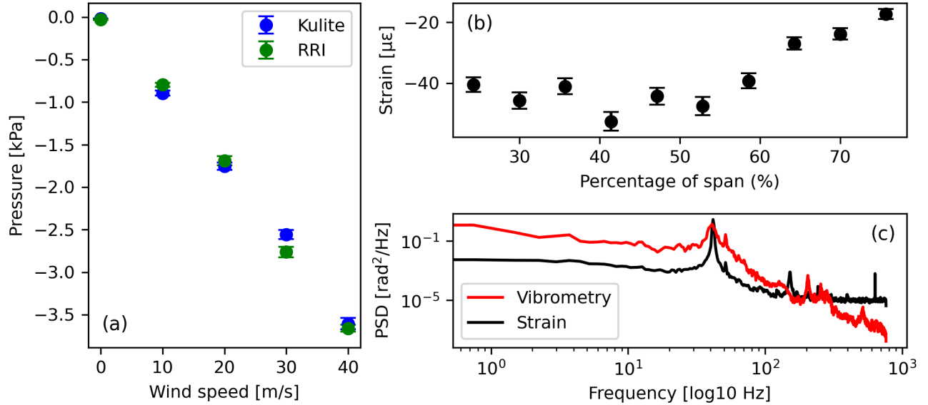
Figure 2. Plots from the ramped wind tunnel test for the measured parameters where (a) shows a comparison between the RRI interrogated optical pressure sensor and Kulite at set wind speeds, (b) the strain distribution for the centre of each segment on the flap at a wind speed of 40 m/s (b), and (c) the frequency analysis from strain and vibrometry data on the flap at 48% span for a wind speed of 40 m/s. All error bars are one standard deviation
