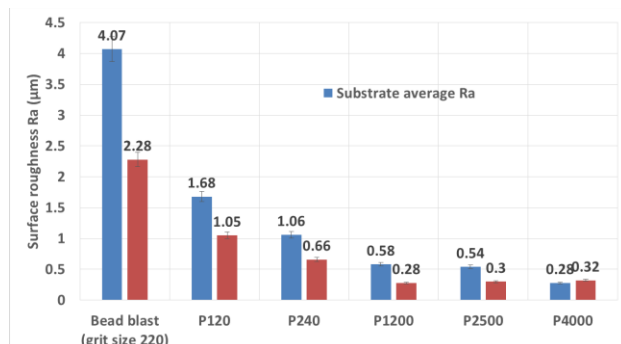
Figure 4. Coating roughness comparison (Ra) – note that the best that can be achieved in around 0.3 µm. Error bar indicates the maximum and minimum measurement per surface profile.
