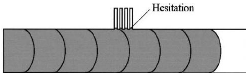
Fig. 2 Hesitation effect in high-aspect-ratio micro-cavities [20]
