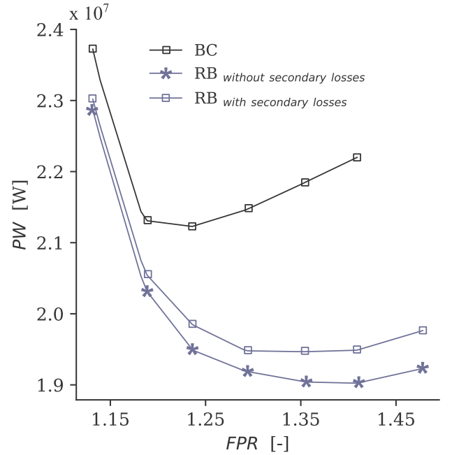
Fig. 10. Effects of secondary and annular losses over power required by the fan at different fan pressure ratios.
