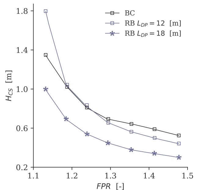
Fig. 11. Capture sheet height for baseline and rotor band configurations at different fan pressure ratios.
