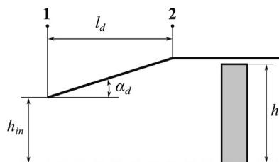
Fig. 4. Intake configuration for baseline (left) and rotor band (right) cases.
