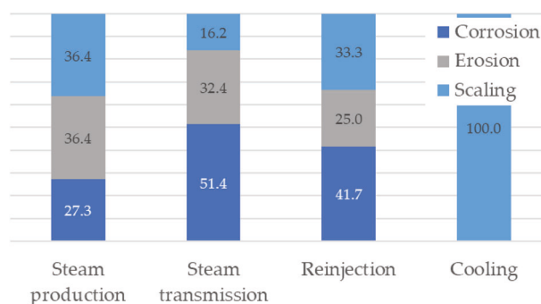
Figure 5. Probability (%) of occurrence of corrosion, erosion, and scaling mechanisms in the main four systems of a geothermal power plant, obtained as a summary of the table in ref. [32], where critical components, principal damage mechanisms and their effects compiled from FMEA analysis from 12 different geothermal power plants were analyzed.
