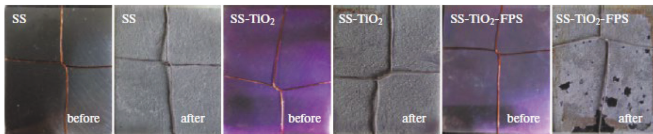
Figure 38. Surface photographs of the un-coated 304 stainless steel coupons and coated coupons before and after immersion for 720 h in simulated geothermal water at 80 °C. Reproduced with permission. [172] Copyright 2018, Springer.
