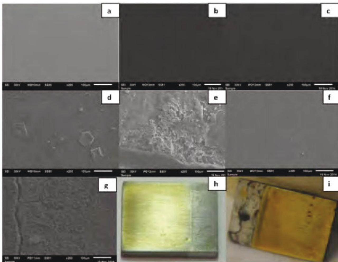
Figure 16. SEM micrographs before and after exposure tests of polybenzoxazine (PBZ) and rubber-modified (PBZ-R)/montmorillonite (MMT) nanoclay composites: a) bare carbon steel, b) PBZ-R, c) PBZ-R-5MMT before immersion in geothermal brine, d) bare steel immersed in 0.5 M NaCl, e) bare steel, f) PBZ-R, g) PBZ-R-5MMT immersed in geothermal brine for 7 days, and optical images of PBZ-R-5MMT, h) before immersion, i) after immersion in simulated geothermal brine for 7 days. The smooth surface appearance of the sample PBZ-R-5MMT in panel (i) shows no clear signs of corrosion or damage. Reproduced with permission. [97] Copyright 2019, Association for Materials Protection and Performance.
