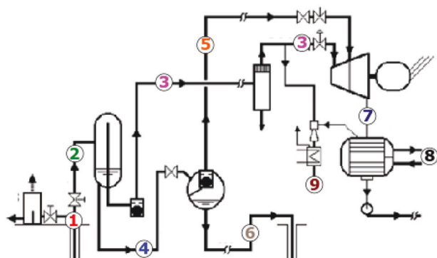
Figure 4. The schematic diagram of the double-flash power plant configuration from Figure 3c [23] adapted with areas of significant geothermal fluid properties variation highlighted with numbers. These properties are reported, for a class III fluid (according to the classification in Table 3), in Table 4. Reproduced with permission. [23] Copyright 2011, Geo-Heat Digital Library, Oregon Institute of Technology Library, Klamath Falls, Oregon.
