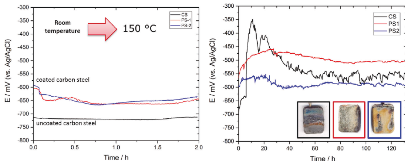
Figure 9. Open Circuit Potential (OCP) of carbon steel, PS1, and PS2 paint systems in artificial geothermal water and oxygen free environment at 150 °C and 1 MPa for 132 hours. Reproduced with permission. [67] Copyright 2019, Association for Materials Protection and Performance.
