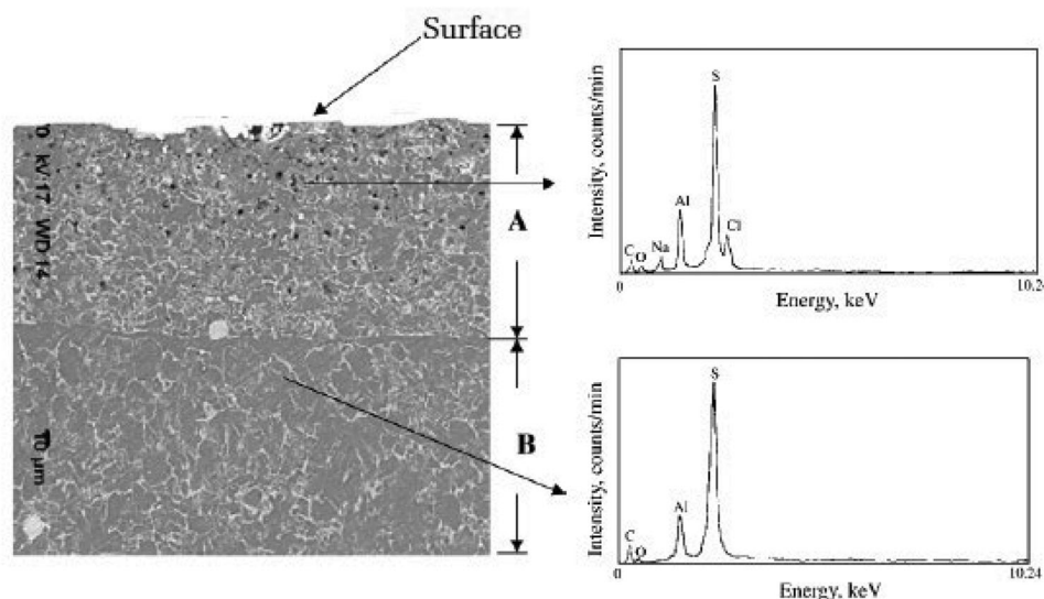
Figure 18. Backscattering SEM image and EDX spectra for the cross-sectional area of 15wt% boehmite-filled PPS paint system after exposure for 15 days in 300 °C brine. Porosity is generated within the paint layer in contact with the exposure medium, which was linked to an excessive amount of boehmite phase. Reproduced with permission. [113] Copyright 2004, SAGE Publications Inc.
