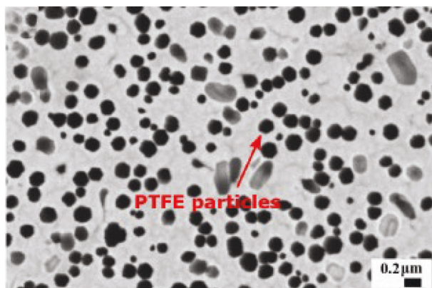
Figure 34. Sem micrograph of electroless plated Ni-P-PTFE layer as reported by Fanicchia et al. Reproduced with permission. [143] Copyright 2021, International Geothermal Association.
