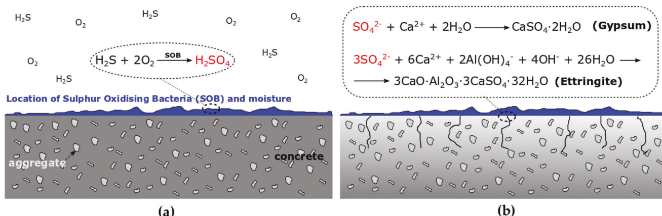
Figure 11. Microbiologically Induced Corrosion (MIC) of concrete due to sulfur oxidising bacteria (SOD) is due to the formation of a) sulfuric acid ( H_2SO_4 ) from hydrogen sulfide ( H_2S ) and oxygen ( O_2 ) in the atmosphere and b) sulfuric acid attack with formation of hydrated gypsum and ettringite compounds, causing substrate cracking and disintegration.
