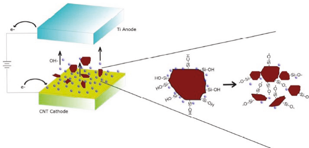
Figure 24. Graphical description of proposed electrochemically induced silicate dissolution cleaning mechanism provided by the carbon nanotubes(CNT)/polyvinylalcohol(PVA) paint for the membrane distillation (MD) process. Reproduced with permission. [126] Copyright 2017, American Chemical Society.
