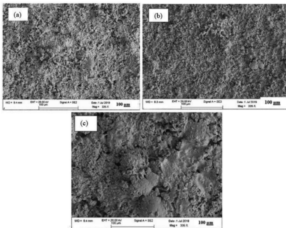
Figure 30. Surface SEM micrographs of the HVOF-deposited cermet coatings, tested against sliding wear behavior by Boakye et al.: a) WC-Co-Cr, b) \text{Cr}_3\text{C}_2 -NiCr, and c) CA3 – Ni-Cr-Fe-Si-B-C. Reproduced with permission. [144] Copyright 2021, International Geothermal Association.
