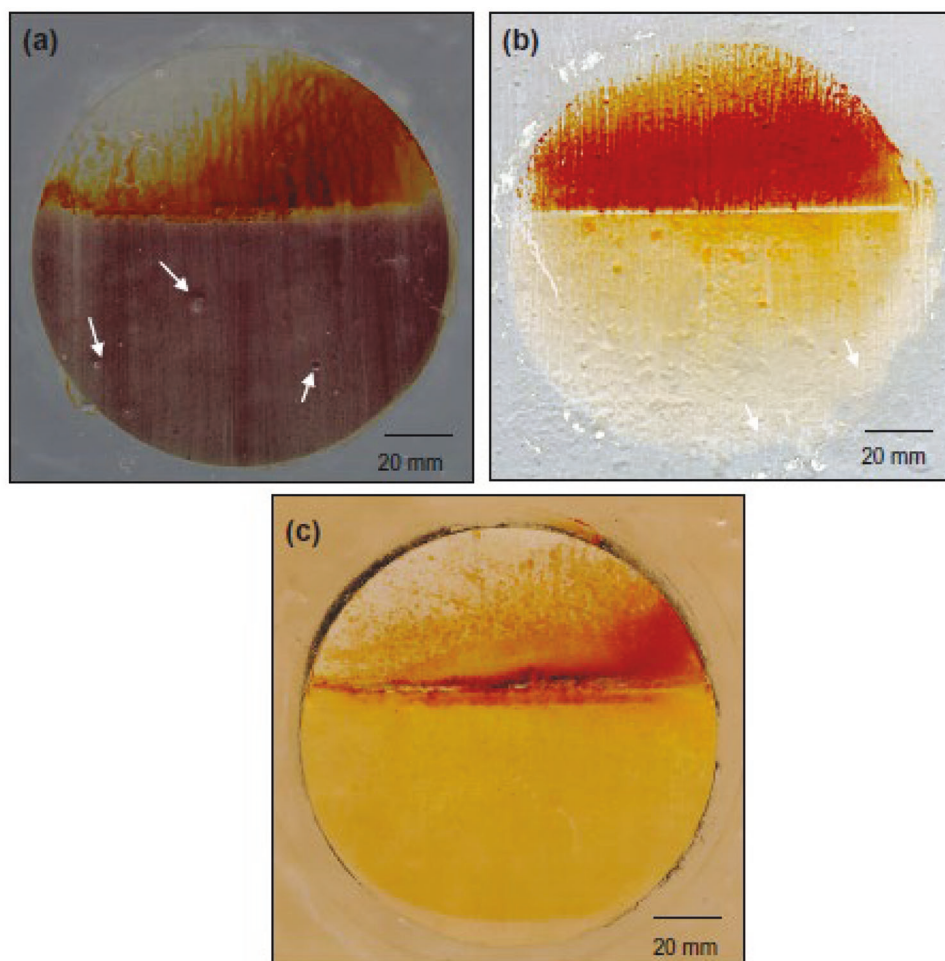
Figure 12. Appearance of a) Amercoat 351, b) Amercoat 385, c) Sikagard 62 after 60-day exposure to T. ferrooxidans . All the epoxy coatings show good condition, except for Amercoat 351 where blisters were observed (white arrows). Reproduced with permission. [80] Copyright 2011, Elsevier.
