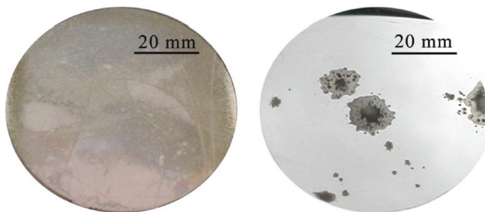
Figure 28. Surface photographs of (left) BP-coating and (right) 304 L stainless steel after potentiodynamic polarization test in 5.7 M NaCl solution at 25 °C. Pitting is observed on the un-coated stainless-steel substrate. Reproduced with permission. [135] Copyright 2014, Elsevier.
