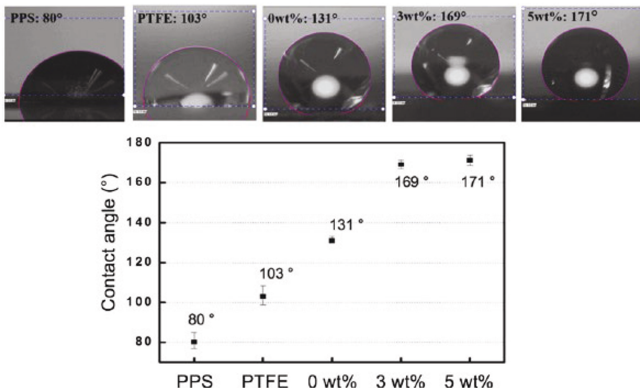
Figure 20. Water contact angle measured for PPS, PPS/PTFE and PPS/PTFE/MWCNT paint systems at different MWCNT loading levels. Reproduced with permission. [121] Copyright 2016, Wiley-VCH GmbH.
