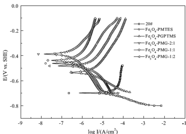
Figure 23. Potentiodynamic polarization curves of different ferric oxide polysiloxane-based composite coatings in 3.5 wt.% NaCl solution. The best performance was demonstrated by specimen \text{Fe}_3\text{O}_4\text{-PMG-2:1} . Reproduced with permission. [125] Copyright 2017, Elsevier.
