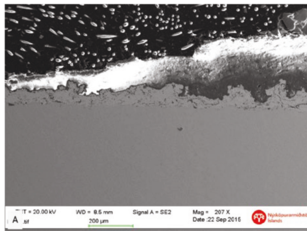
Figure 36. Cross-sectional SEM micrograph of \text{Al}_2\text{O}_3/\text{TiO}_2 coating after 38 days in-situ exposure at the Hellisheiði power plant (Iceland), showing no cracks nor delamination, but significant erosion wear. Reproduced with permission. [141] Copyright 2017, Association for Materials Protection and Performance.
