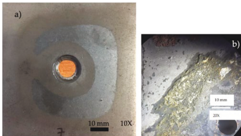
Figure 41. Surface photographs of a) \text{TiB}_2\text{-Ni}_3\text{B} nanocomposite coating and b) uncoated stainless-steel type 304 specimens after 1 month in situ exposure to geothermal fluid at the Geothermal Unit Los Hornos (Mexico); no clear corrosion products are visible on the coated coupon as opposed to the steel substrate. Reproduced with permission. [183] Copyright 2021, Institute of Physics.
