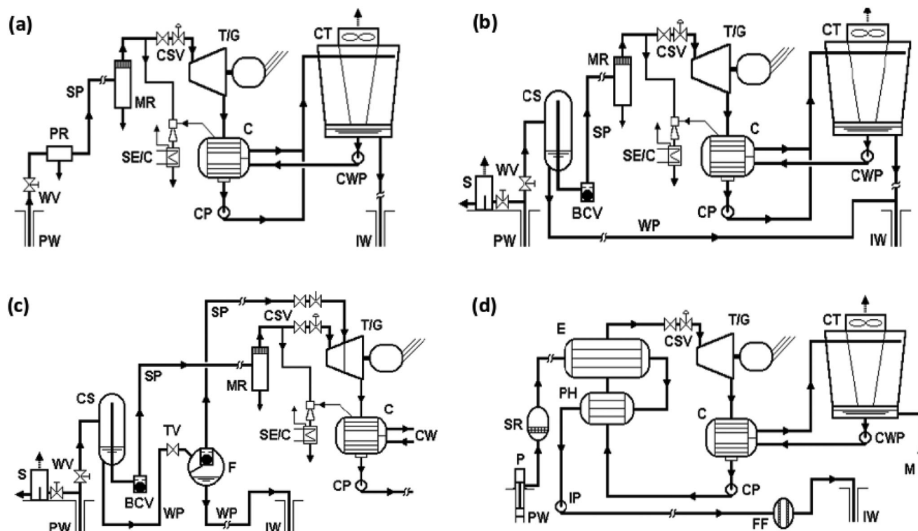
Figure 3. Schematics of geothermal power plant configurations: a) dry steam, b) single-flash, c) double-flash, and d) binary. In the figure: BCV (ball check valve), CP (condensate pump), CSV (control and stop valve), CW (cooling water), E (evaporator), FF (final filter), IW (injection wells), MR (moisture remover), PH (preheater), R (recuperator), SE/C (steam ejector/condenser), SP (steam piping), T/G (turbine/generator), WP (water piping), C (condenser), CS (cyclone separator), CT (cooling tower), CWP (cooling water pump), F (flasher), IP (injection pump), M (make-up water), P (well pump), PR (separator), PW (production wells), S (silencer), SH (superheater), SR (sand remover), TV (throttle valve), WV (wellhead valve). Reproduced with permission. [23] Copyright 2011, Geo-Heat Digital Library, Oregon Institute of Technology Library. Klamath Falls, Oregon.
