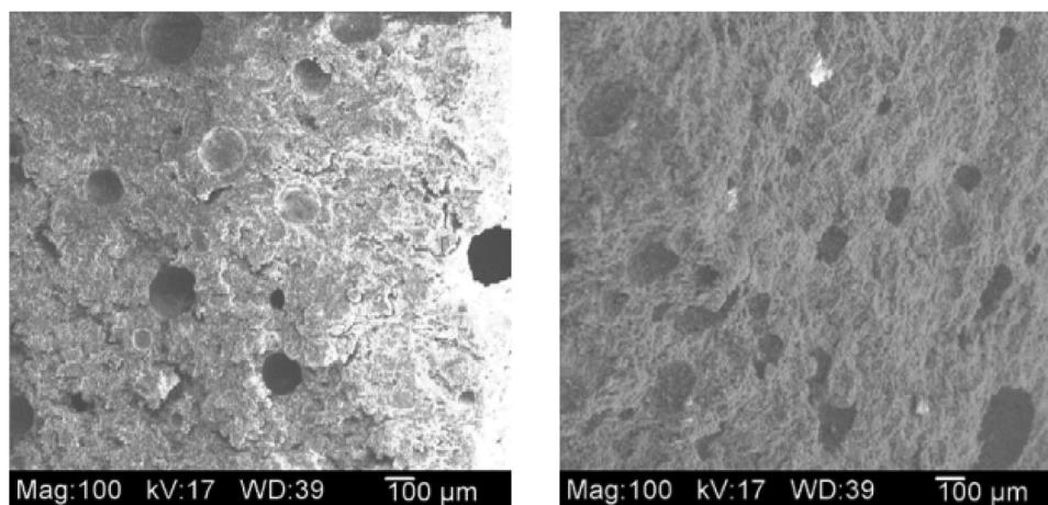
Figure 7. SEM micrographs of fractured surfaces for styrene acrylic latex (SAL)/calcium aluminate cement (CAC) at 30/70 ratio in (left) non-exposed and (right) exposed to 21 days simulated geothermal conditions. Pores originally identified on the as-deposited specimen (left) were observed to be filled with boehmite and calcite phases during the exposure (right). Reproduced with permission. [64] Copyright 2006, Brookhaven National Laboratory.
