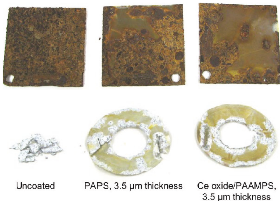
Figure 22. Uncoated, undoped PAPS and Ce oxide/PAAMPS-coated carbon steel coupons (top) and aluminum fins (bottom) after the 24 500-cycle test, showing significant improvements in corrosion performance for the latter. Reproduced with permission. [124] Copyright 2006, Geothermal Rising.
