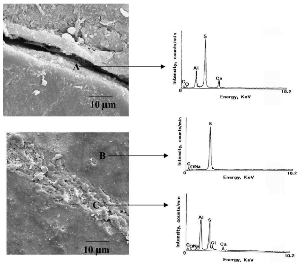
Figure 19. SEM images coupled with EDX spectra for cleaved PPS coatings with 5 wt.% CA fillers before (top) and after (bottom) exposure for 24 h to CO 2 -laden brine at 200 °C, clearly indicating that crack filling with block-like crystals has occurred. Reproduced with permission. [115] Copyright 2003, Elsevier.
