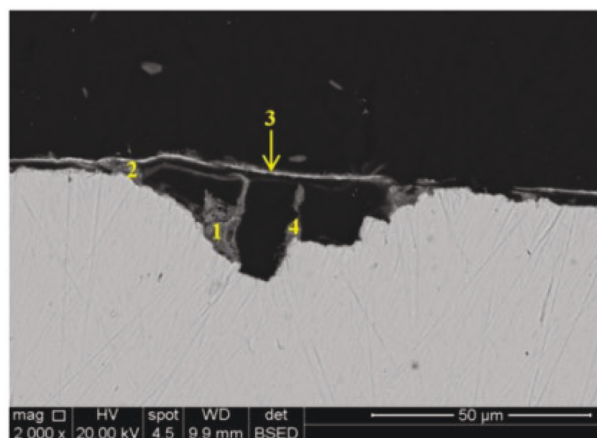
Figure 27. SEM micrograph of a corrosion pit formed under antimony-coated carbon steel coupon after exposure to aerated pH 5.4 solution. Reproduced with permission. [133] Copyright 2015, International Geothermal Association.
