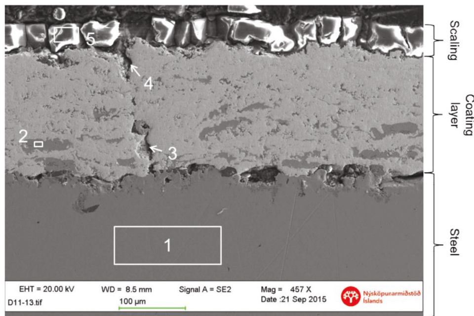
Figure 29. Cross-sectional SEM micrograph of HVOF WC-Co-Cr cermet coating deposited onto carbon steel, showing vertical cracks and voids at the interface after in-situ exposure test at the Hellisheiði geothermal power plant. Reproduced with permission. [141] Copyright 2017, Association for Materials Protection and Performance.
