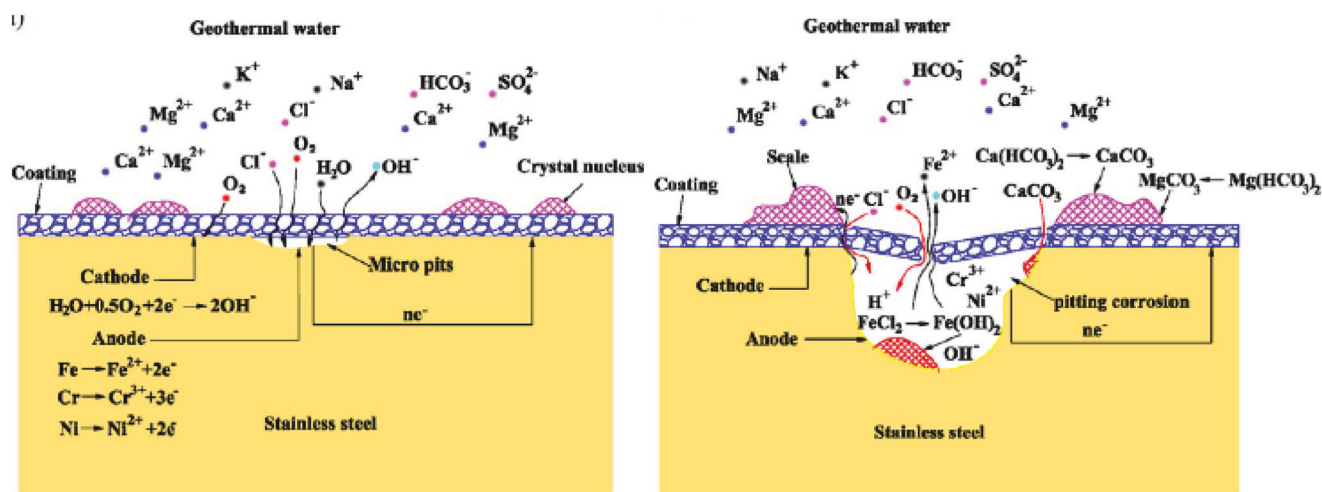
Figure 39. Schematic representation of corrosion and scaling mechanisms proposed by Cai et al. involving composite \text{ZrO}_2\text{-TiO}_2 coatings deposited onto AISI 304 stainless steel and exposed to NaCl-rich simulated geothermal water at 20 °C. a) The tortuous path of \text{O}_2 and \text{Cl}^- through the protected coating at the initial stage and b) coating damage and scale formation processes after prolonged immersion time. Reproduced with permission. [174] Copyright 2016, American Chemical Society.
