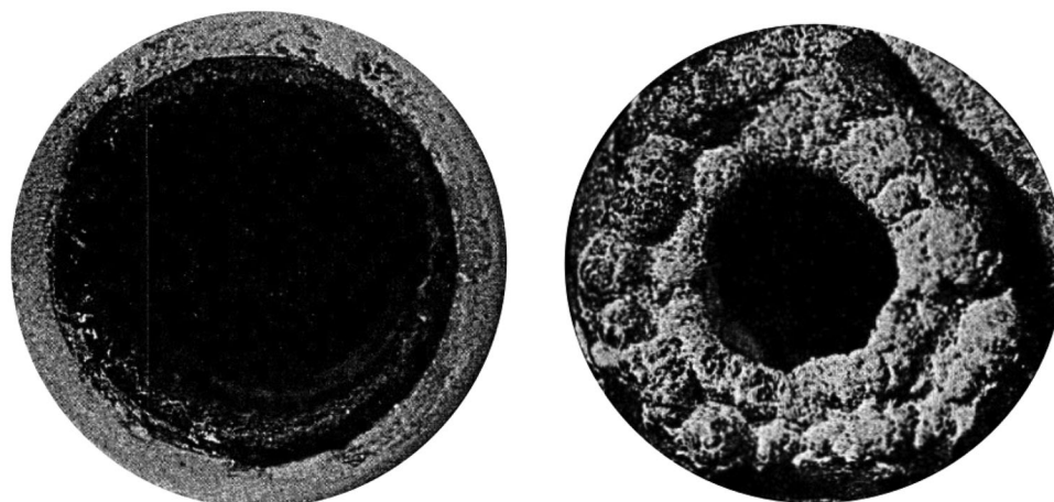
Figure 13. Teflon PFA (left) and Ployphenylquinoxaline (right) nozzle exits after field tests showing considerable difference in amount of mineral scaling. The Teflon PFA paint system demonstrated the least scaling and highest resistance to erosive wear among the tested systems by Lorensen et al. Reproduced with permission. [63] Copyright 1975, Lawrence Livermore National Laboratory.
