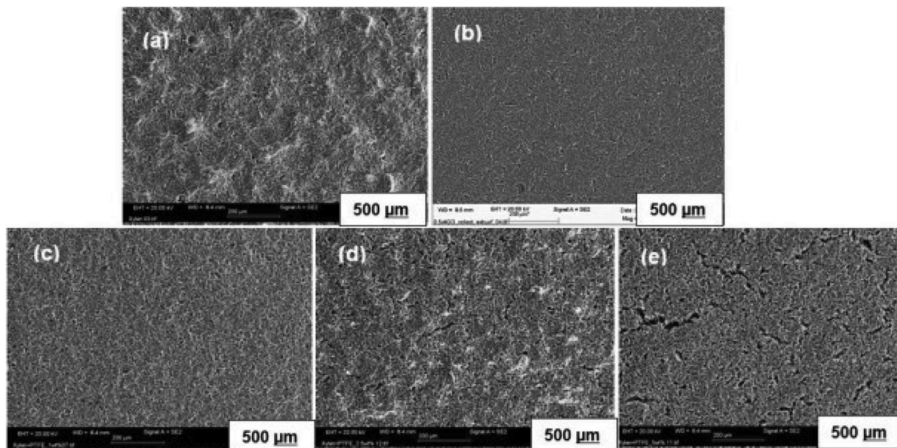
Figure 15. SEM micrographs of the surface of Xylan-based coatings a) pure Zylan, b) Xylan+0.5 wt.%Graphene Oxide(GO), c) Xylan+1 wt.%GO, d) Xylan+2.5 wt.%GO, e) Xylan+5 wt.%GO. Reproduced with permission. [94] Copyright 2021, International Geothermal Association.
