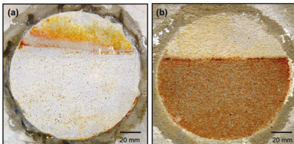
Figure 40. Surface photograph of a) Sikagard 75 EpoCem mortar and b) latex-modified mortar after exposure to Thibacillus ferrooxidans showing very slight etching in immersed zone. Reproduced with permission. [80] Copyright 2011, Elsevier.
