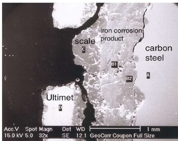
Figure 35. SEM micrograph of Ultimet-coated (Co-based alloy) carbon steel coupons after exposure for 1200 h within a wellhead in the Salton Sea geothermal area. Scale and corrosion products are observed at the interface between coating and substrate because of brine permeation through defects in the coating. Reproduced with permission. [146] Copyright 2002, Geothermal Rising.
