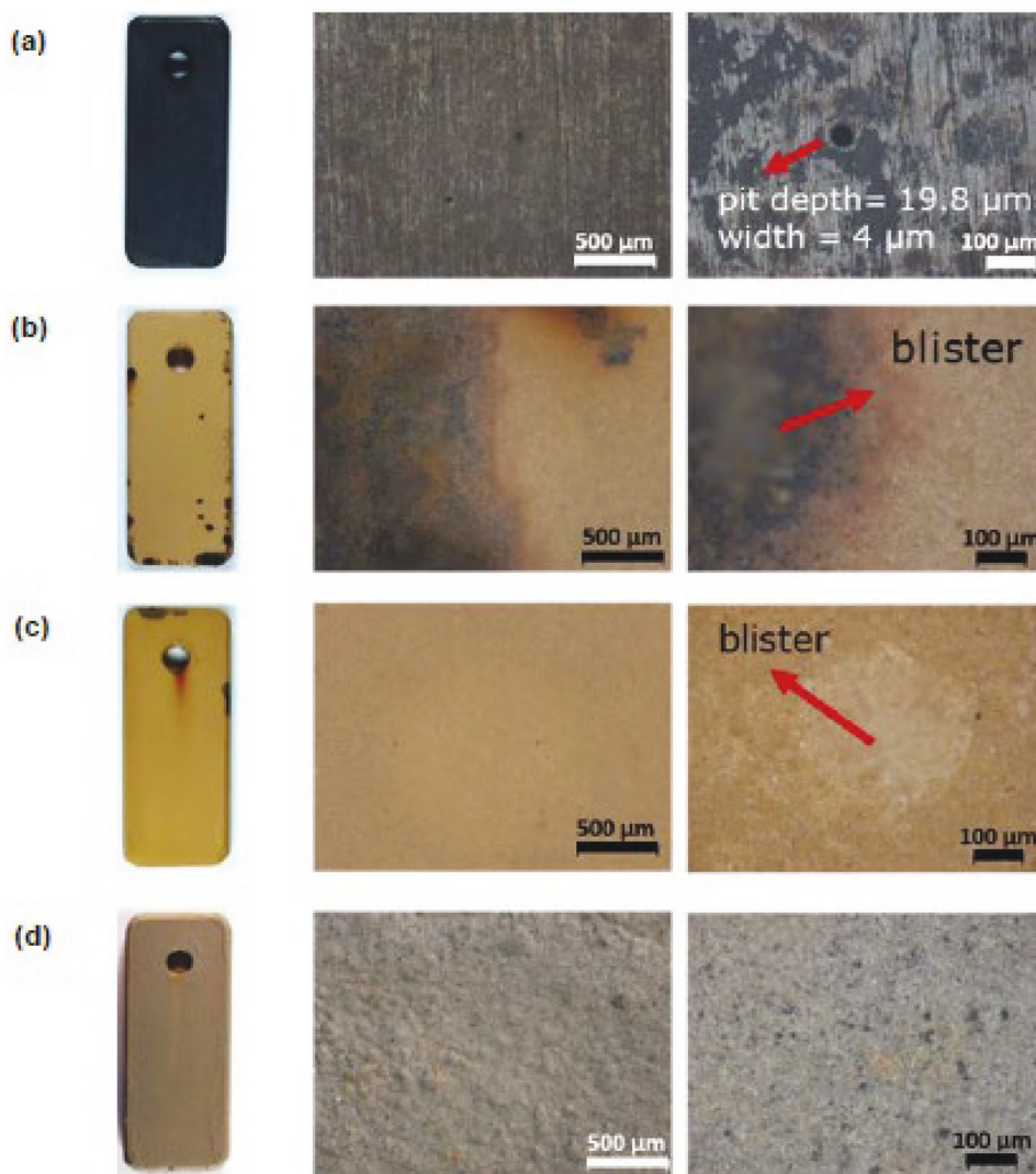
Figure 8. Overview (left), stereo picture (center), and light microscope images (right) of specimens exposed at 150 °C and 1 MPa for 7 days of a) carbon steel, b) binder, c) Si15, and d) PS. Reproduced with permission. [66] Copyright 2018, Association for Materials Protection and Performance.
