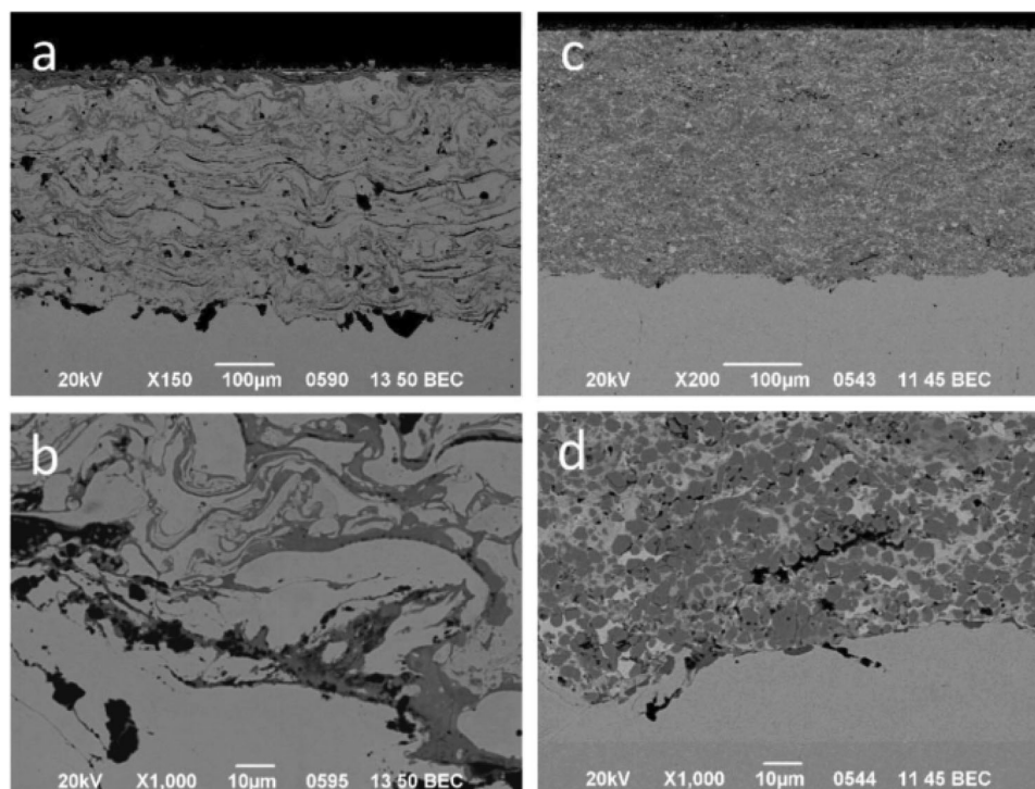
Figure 33. Cross-sectional SEM micrograph of a,b) TWAS-deposited \text{Cr}_{13}\text{Fe}_{87} and c,d) HVOF-deposited \text{Ce}_2\text{C}_3 -NiCr (cermet) coatings after 3 months exposure to simulated geothermal fluid. Corrosion damage is observed, particularly with the Fe-based alloy. Reproduced with permission. [142] Copyright 2021, Tanger Ltd.
