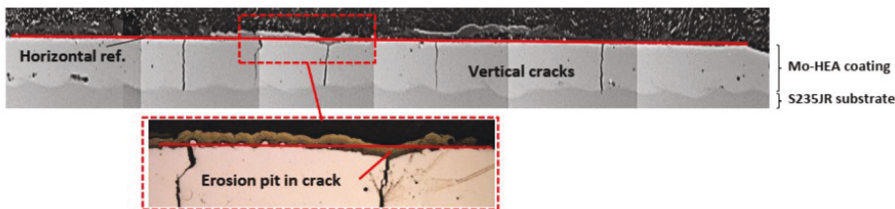
Figure 32. The laser metal deposited CoCrFeMo 0.85 Ni coating onto carbon steel revealed manufacturing cracks, which were considered responsible for a locally enhanced erosion damage after erosion in-situ exposure at the Hellisheiði geothermal power plant. Reproduced under the term of CC-BY license. [155] Copyright 2021, The Authors, published by MDPI.
