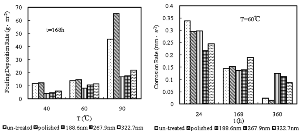
Figure 37. The performance of bare and SiO 2 coated copper substrates, at different coating thicknesses, was assessed against (left) fouling and (right) corrosion performance by Chen et al. Results showed improved fouling performance but corrosion mitigation only at short exposure times, due to worsening of the coating mechanical properties. Reproduced with permission. [168] Copyright 2021, American Chemical Society.
