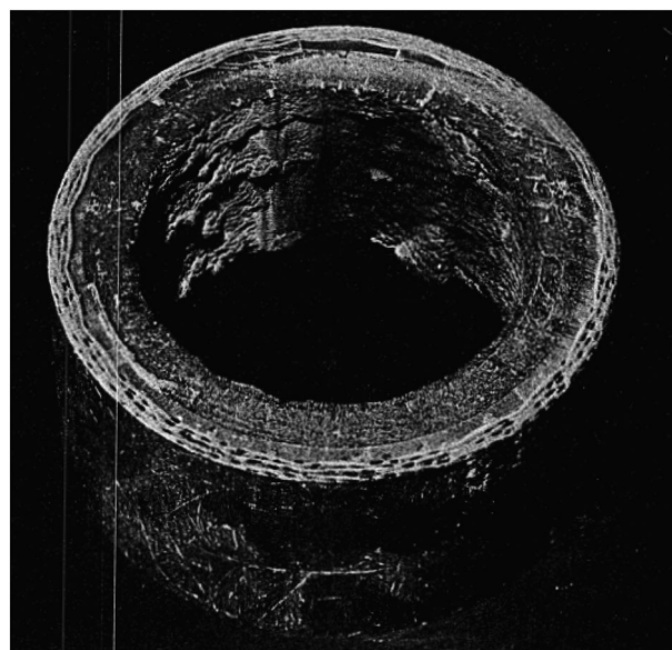
Figure 10. Epoxy fiberglass pipe after 72 h exposure to a synthetic hypersaline brine (24 wt.% NaCl) at 300 °C, showing clear presence of scale on the internal diameter. Reproduced with permission. [63] Copyright 1975, Lawrence Livermore National Laboratory.
