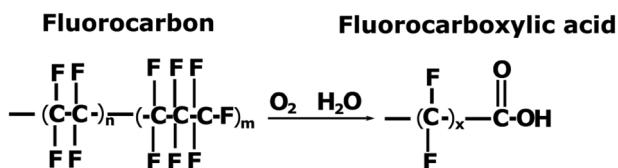
Figure 14. Mechanism of hydrothermal oxidation of the polyfluorocarbon, possibly leading to the formation of fluorocarboxylic acid fragments.
