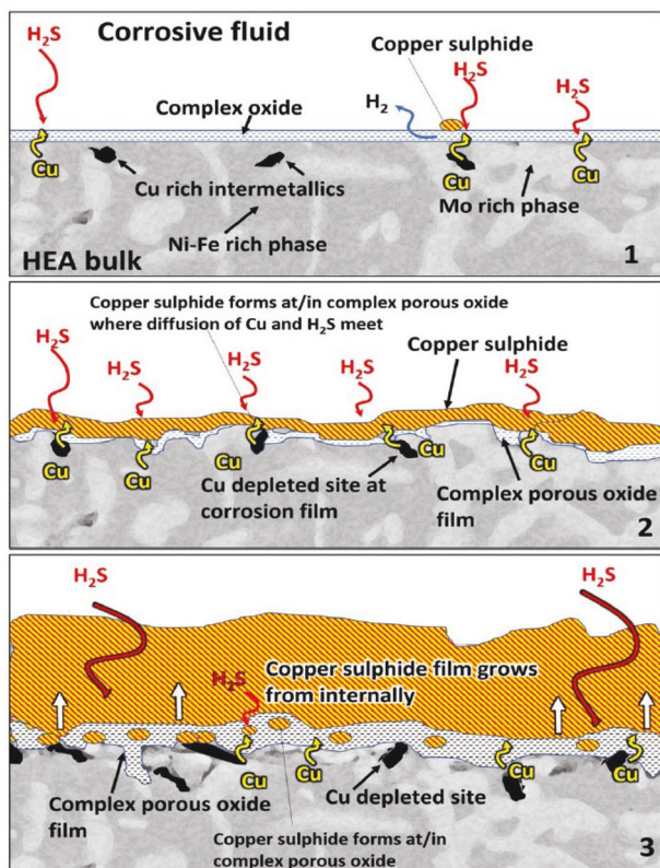
Figure 31. \text{Cu}_2\text{S} formation mechanism proposed by Thorhallsson et al., for Cu-containing HEAs after exposure to hot geothermal brine resembling the IDDP1 chemistry (Krafla region, Iceland). Reproduced with permission. [152] Copyright 2021, Elsevier.
