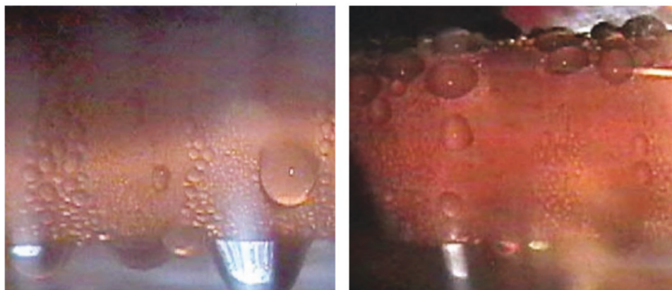
Figure 25. Surface photograph of condensation onto a self-assembled monolayer paint-coated tube (SAM-2) after 100 h (left) and 3600 h test (right), demonstrating an increase in drop size with exposure time. Reproduced with permission. [128] Copyright 2006, Geothermal Rising.
