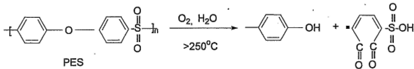
Figure 17. As suggested by Sugama, [102] hydrothermal oxidation of polyethersulfone (PES) exposed to artificial brine at temperatures >250 °C leads to the formation of hydroxyl and carbonyl groups, with consequent enhancement of moisture susceptibility. Reproduced with permission. [102] Copyright 2005, Brookhaven National Laboratory.
