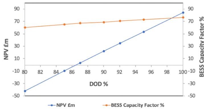
Fig. 10. Impact of DOD on NPV and capacity factor (Optimised)
