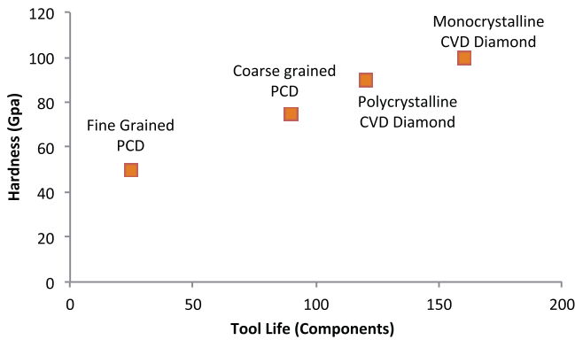
Fig. 5. Evidence of the potential for tool life increase through use of harder tool materials: tool life in turning of metal matrix composite components related to tool hardness (after Cooper et al., 2005).
