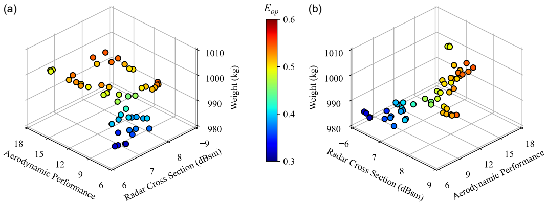
Figure 15. Pareto front of UAV configurations in the ground attack scenario, illustrating the trade-offs among aerodynamic performance, radar cross section and structural weight. The discrete markers represent the Pareto-optimal configurations obtained using the NSGA-II algorithm. The colour map indicates the operational effectiveness ( E_{op} ) of each configuration, evaluated within ground attack mission profiles. To improve the visual interpretation of the three-dimensional trade-off geometry, two different azimuth views are presented: (a) 135° and (b) -135°, to better visualise the three-dimensional trade-off geometry.
