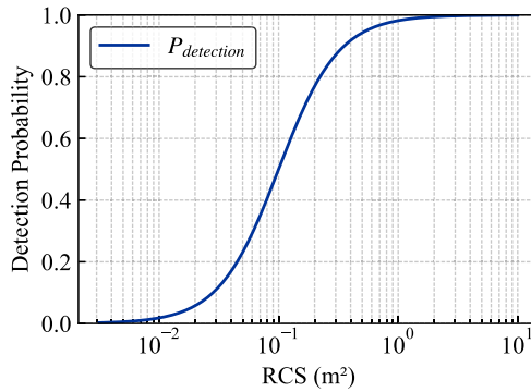
Figure 7. Detection probability curve based on radar cross section (RCS).
