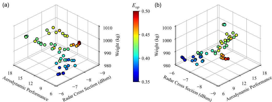
Figure 11. Pareto front of UAV configurations in the aerial combat scenario, illustrating the trade-offs among aerodynamic performance, radar cross section, and structural weight. The discrete markers represent the Pareto-optimal configurations obtained using the NSGA-II algorithm. The colour map indicates the operational effectiveness ( E_{op} ) of each configuration. To improve the visual interpretation of the three-dimensional trade-off geometry, two different azimuth views are presented: (a) 135^\circ and (b) -135^\circ .
