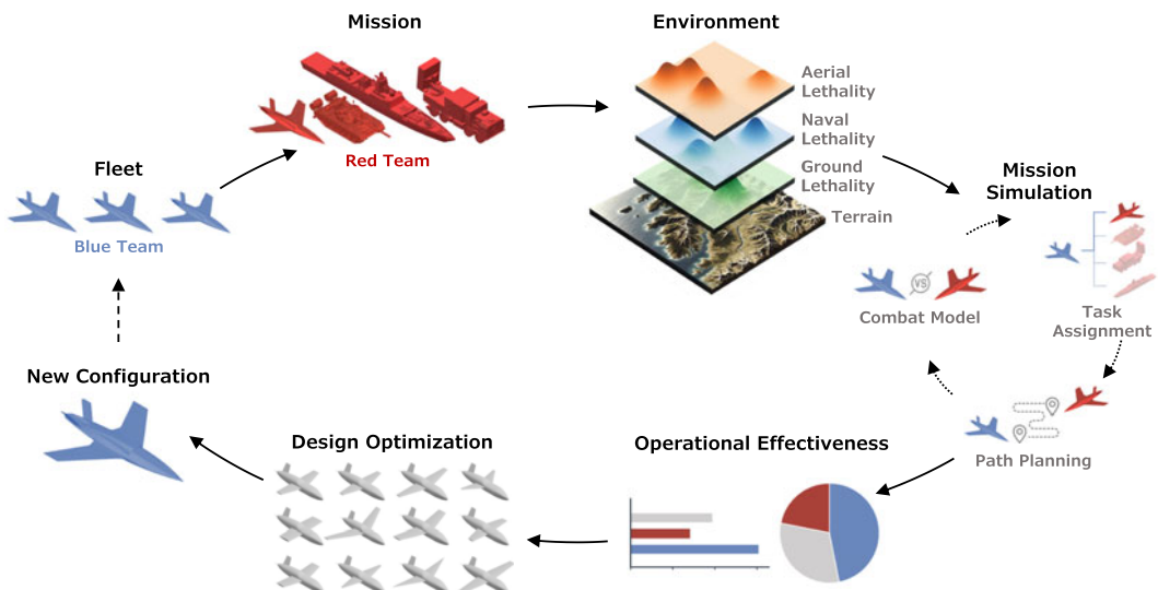
Figure 3. Overview of the mission-centric design optimisation approach for UAVs.
