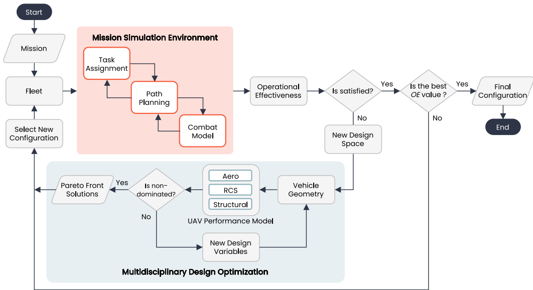
Figure 4. General framework for mission-centric design optimisation process.
