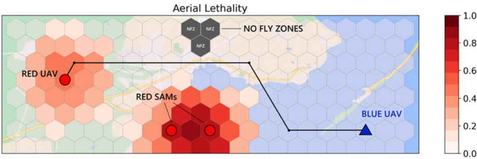
Figure 10. Path planning for UAV in threat zones and NFZs.
