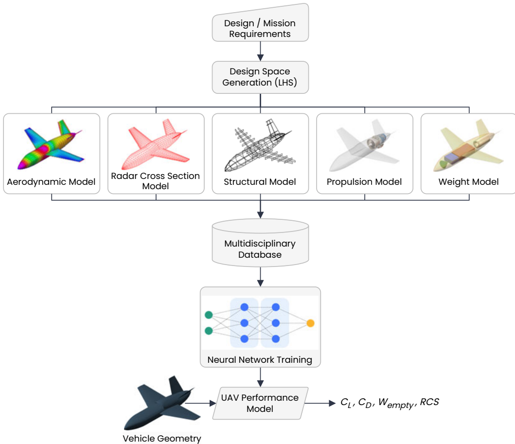
Figure 5. Workflow for generating the ANN-based UAV performance model from multidisciplinary data.
