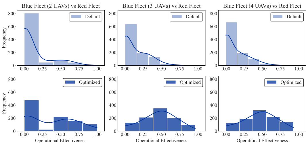
Figure 14. Comparison of operational effectiveness distributions for default and optimised UAV configurations across different Blue Fleet sizes.
