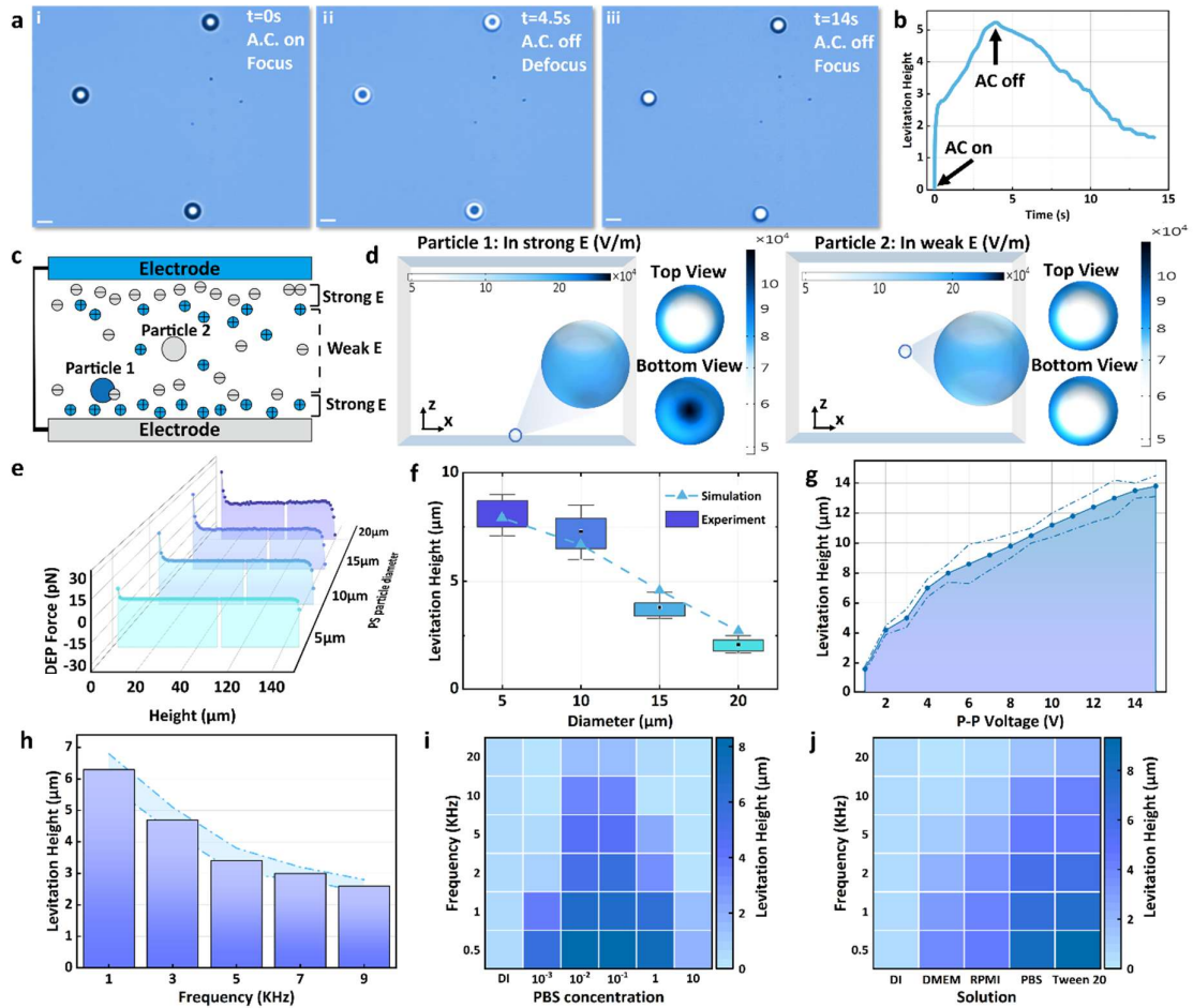
Figure 2. Experimental and simulated characterization of the dielectric levitation mechanism in PS microspheres (a) Levitation and deposition process of three PS microspheres. Scale bar: 10 \mu m . (b) Levitation height versus time for the three PS microspheres. (c) Schematic of electrode polarization in the electric field, with Particle 1 located near the electrode and Particle 2 positioned farther away. (d) Simulated electric field strength distribution for two 10 \mu m PS particles under strong and weak field conditions. Insets display the isometric perspective along with the top and bottom views of the particles. The color bar represents the electric field modulus. (e) Simulated DEP forces for four PS microparticle sizes, highlighting heights near the top and bottom electrodes. (f) Experimentally measured and simulated levitation heights for four particle sizes. All simulations and experiments were conducted using a 1 kHz, 10 Vpp sinusoidal signal. The spacing between the bottom and top plates was 150 \mu m . (g) Relationship between peak-to-peak voltage and particle levitation height. Color band indicates the error bar. (h) Relationship between frequency and particle levitation height. Color band indicates the error bar. (i) Heat map of particle levitation height versus PBS concentration across the frequency range. (j) Heat map of particle levitation height for different solution types across the frequency range.
