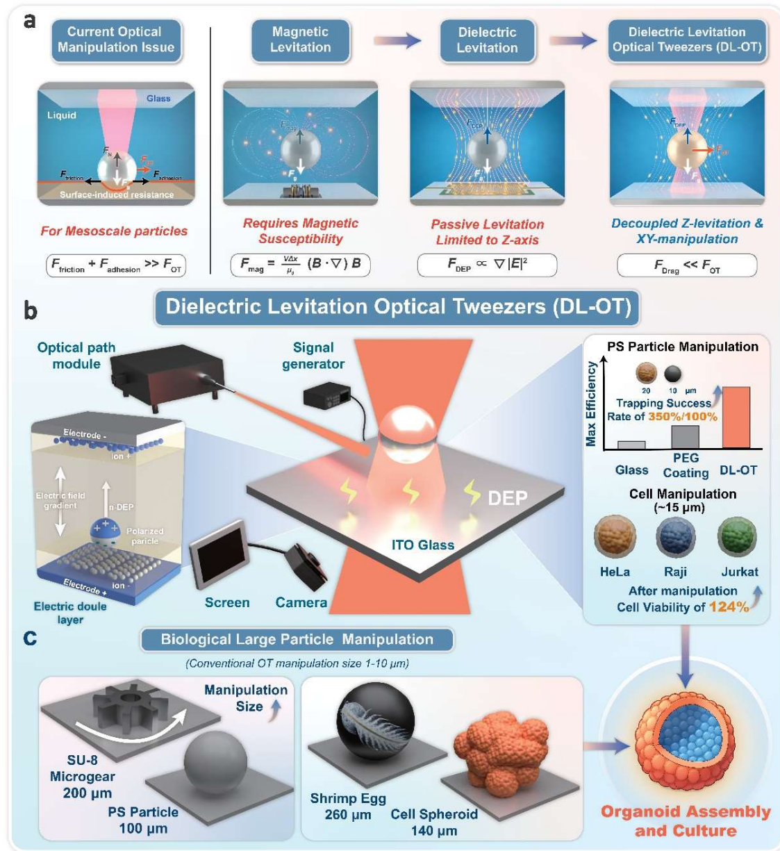
Figure 1. Schematic of Dielectric Levitation Optical Tweezers (DL-OT). (a) Current optical manipulation issue and the inspiration. (b) Schematic of the DL-OT system. The left panel illustrates the n-DEP mechanism within the electric double layer. The middle panel shows the integrated experimental setup. The right panel quantitatively highlights the performance leaps of DL-OT. (c) Demonstration of mesoscale manipulation capabilities, overcoming the conventional 1–10 μm limit to stably transport large objects (100–260 μm), including SU-8 microgears, PS particles, shrimp eggs, and cell clusters, enabling advanced organoid assembly and culture.
